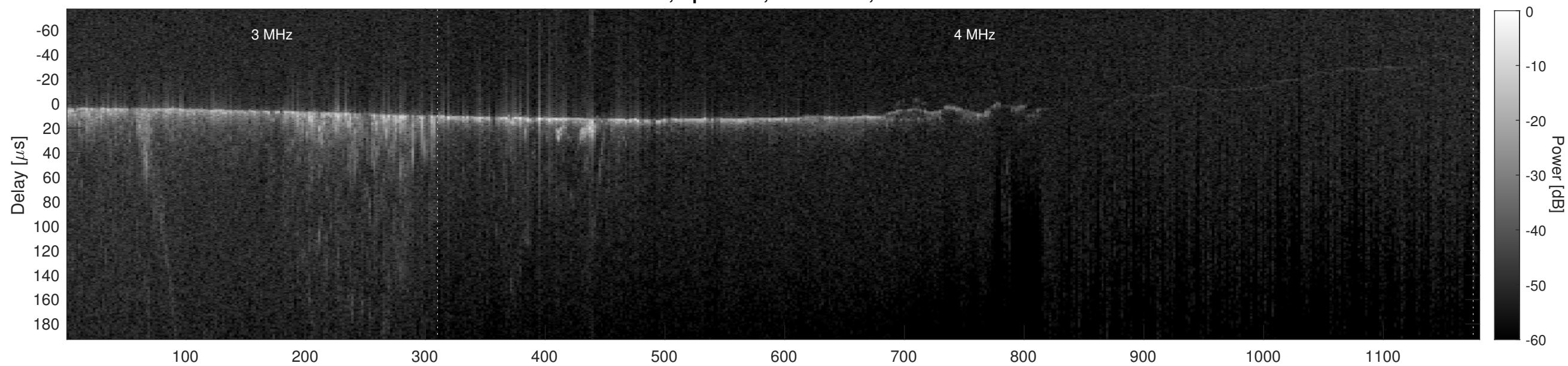
Orbit 9345, Cluttergram
