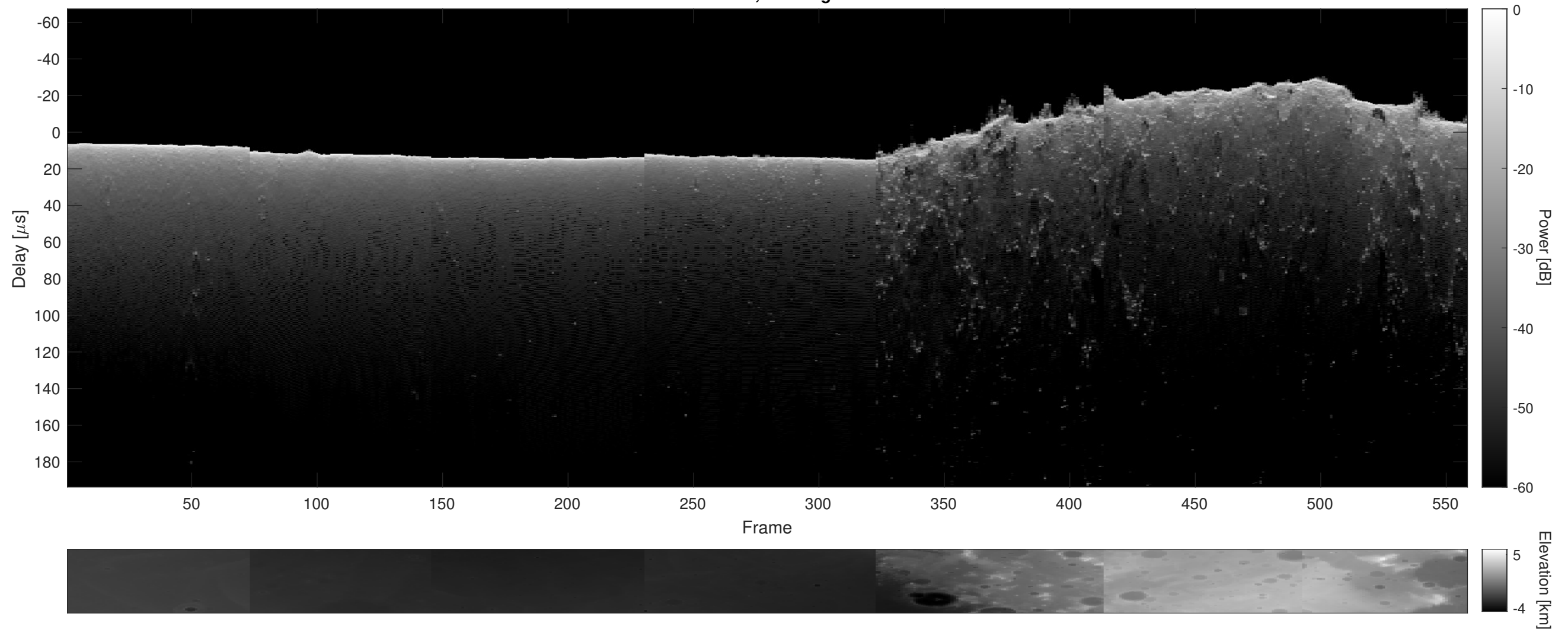
Orbit 9346, Cluttergram
