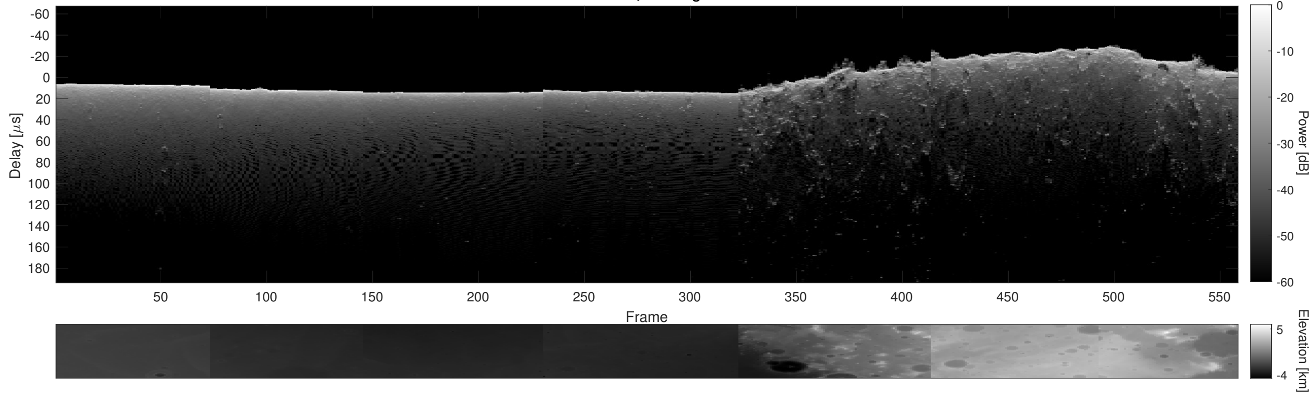
Orbit 9346, Cluttergram
