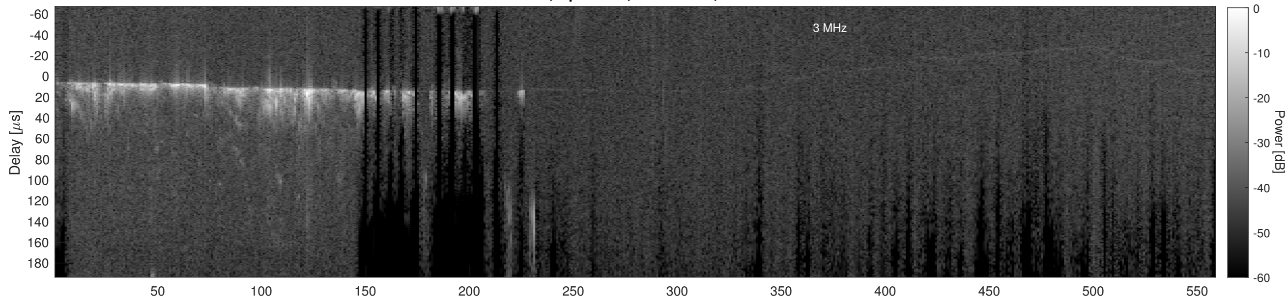
Orbit 9346, Cluttergram
