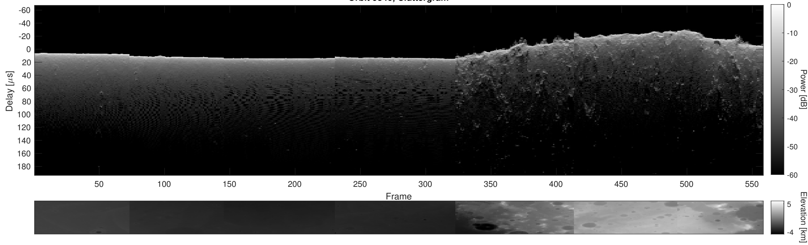
Orbit 9346, Cluttergram
