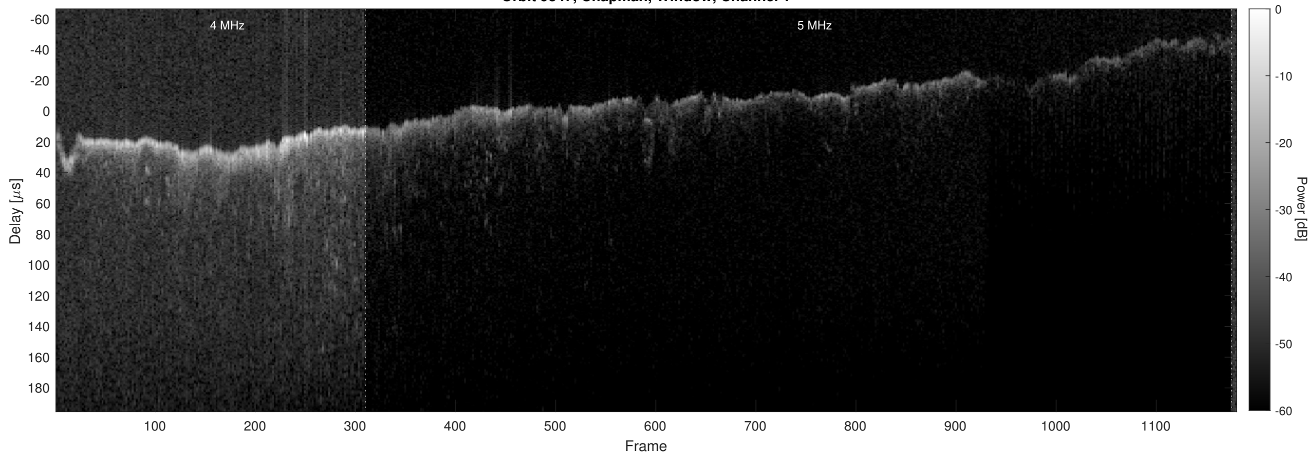
Orbit 9347, Chapman, Window, Channel 2
