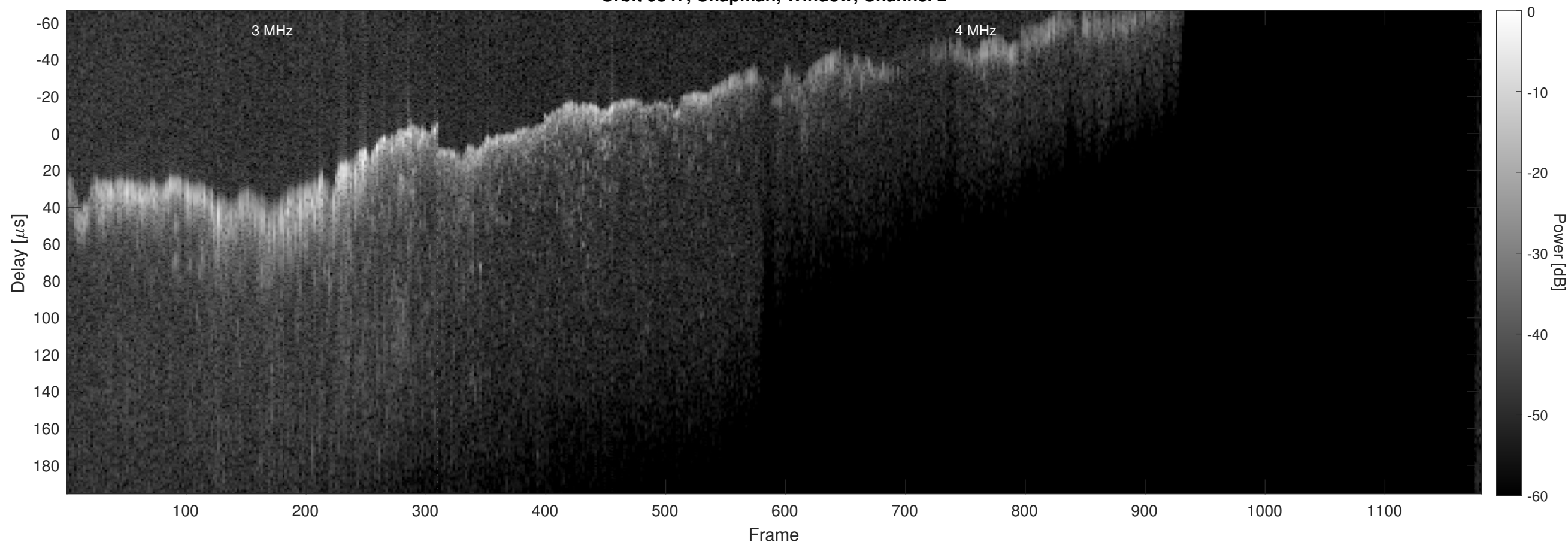
Orbit 9347, Chapman, Window, Channel 2
