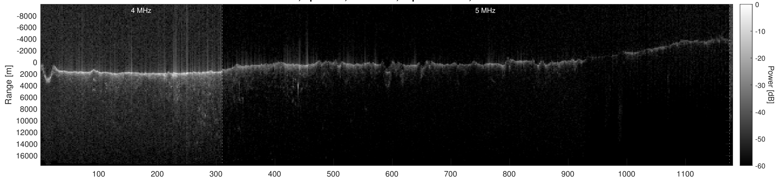
Orbit 9347, Optimized, No Window, Depth-Corrected, Channel 2
