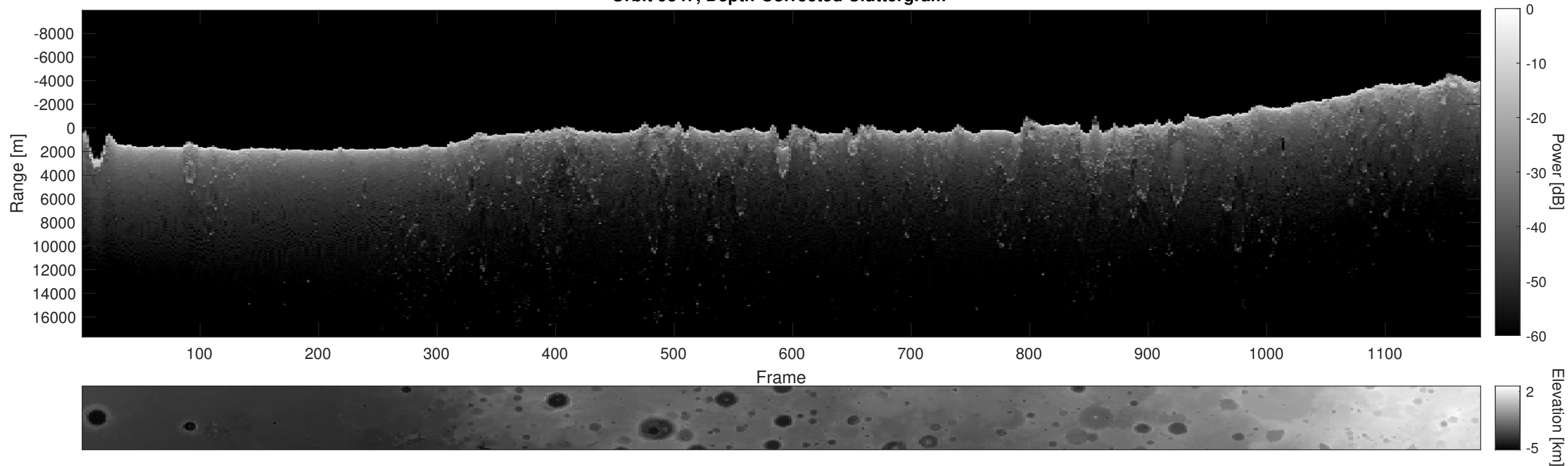
Orbit 9347, Depth-Corrected Cluttergram
