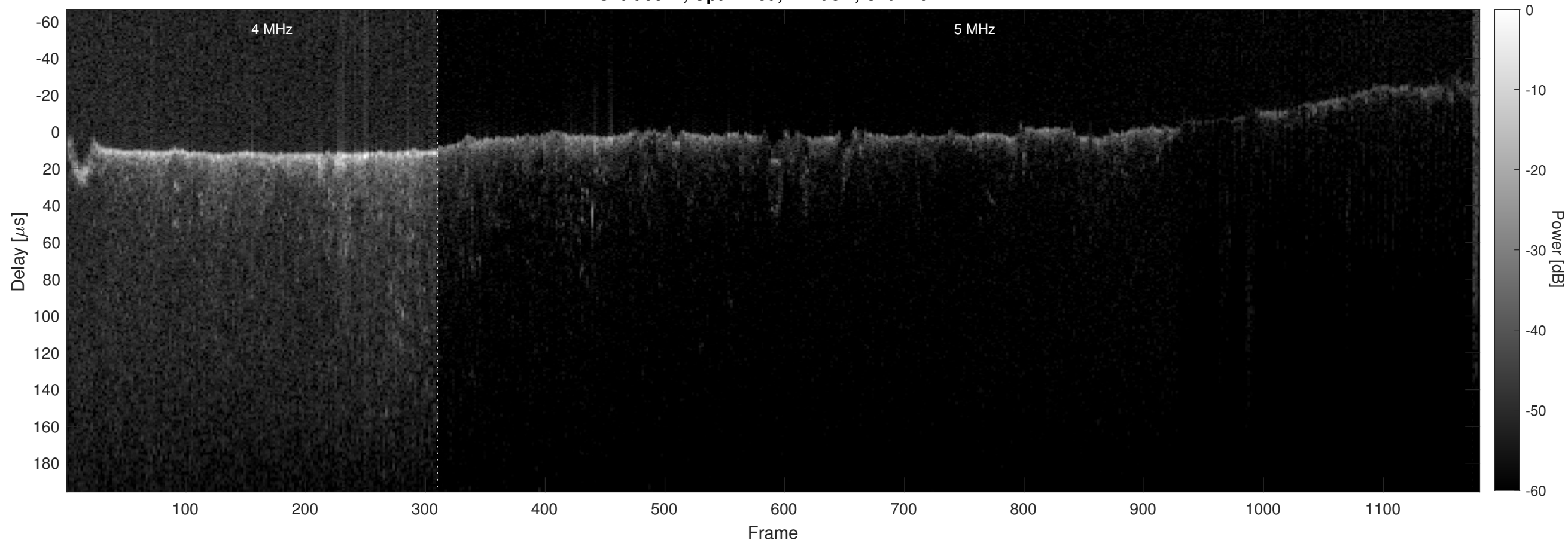
Orbit 9347, Optimized, Window, Channel 2
