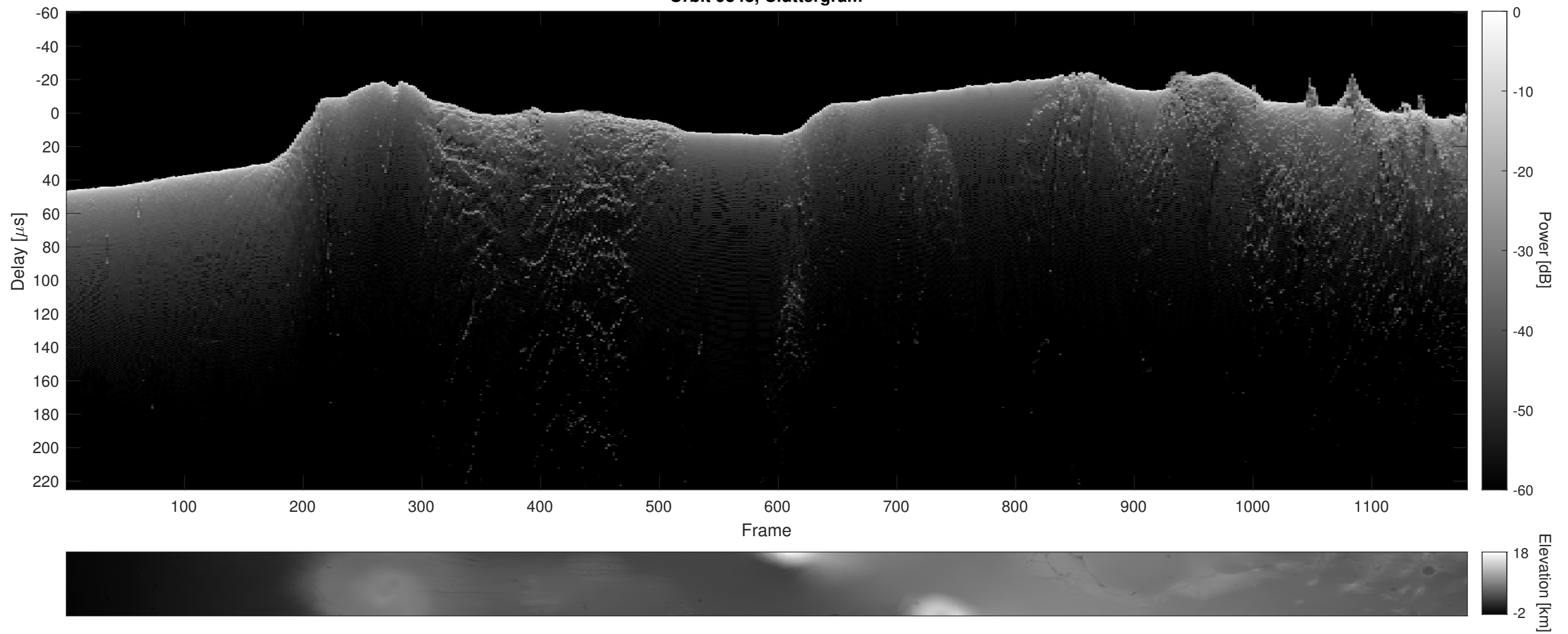
Orbit 9348, Cluttergram
