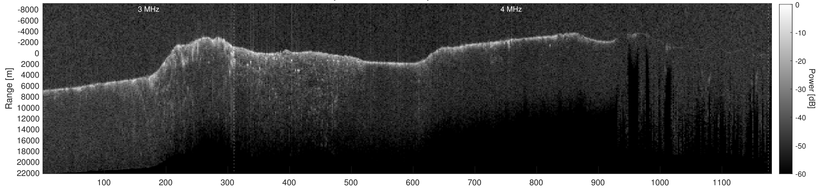
Orbit 9348, Depth-Corrected Cluttergram
