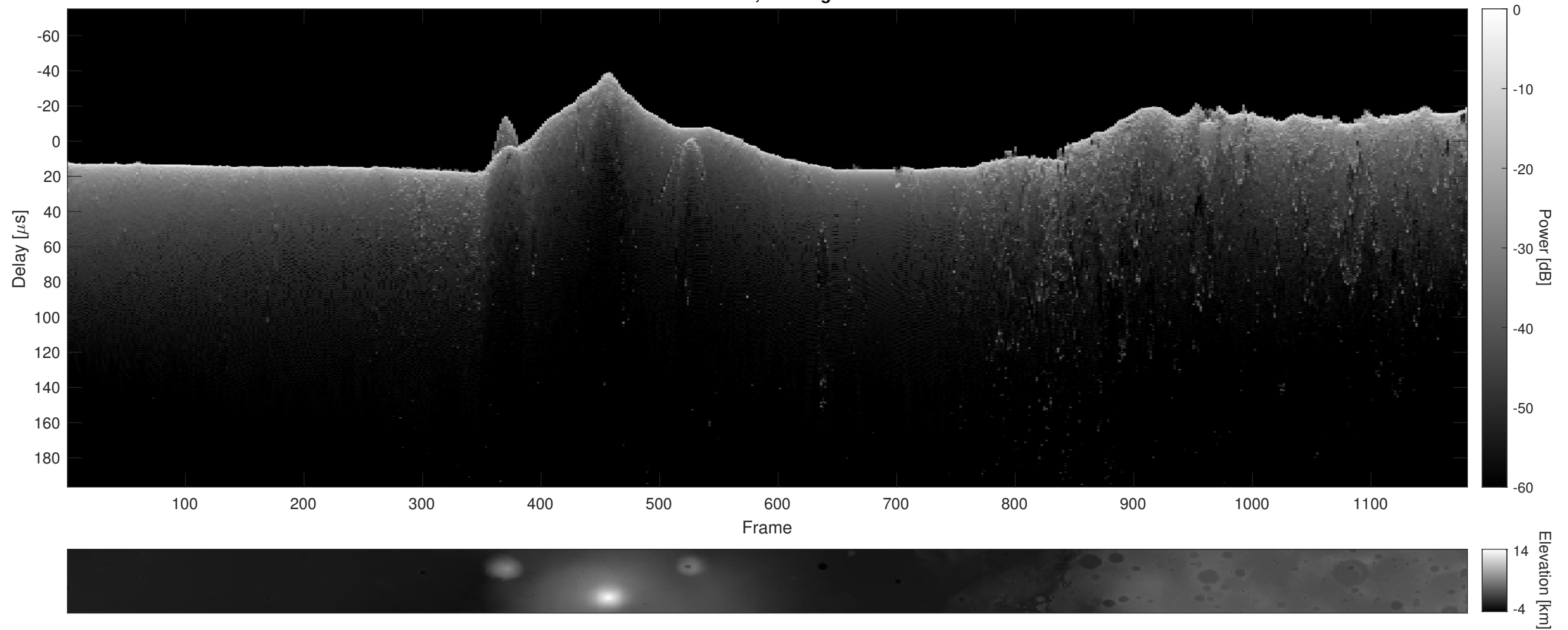
Orbit 9349, Cluttergram
