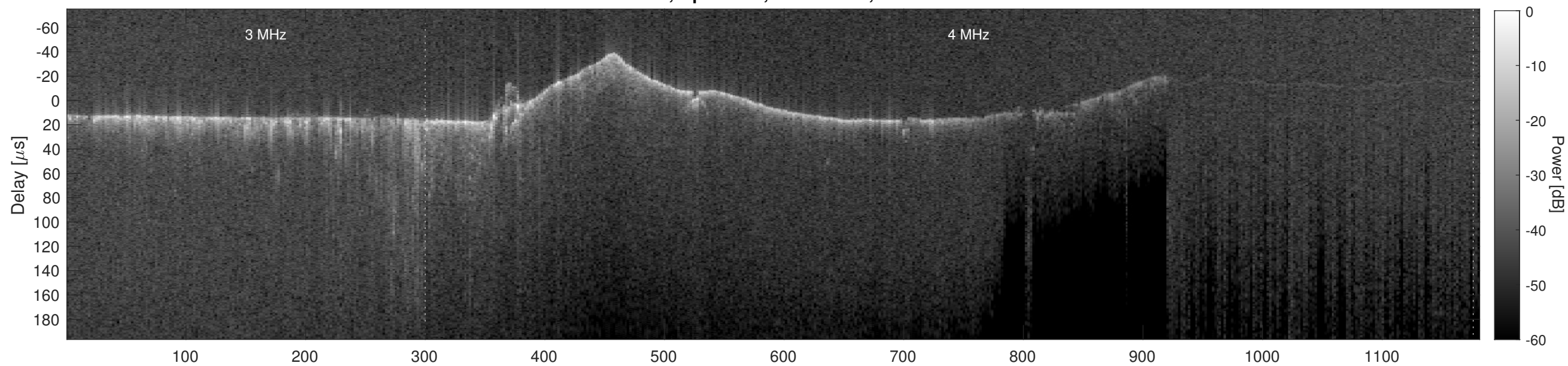
Orbit 9349, Cluttergram
