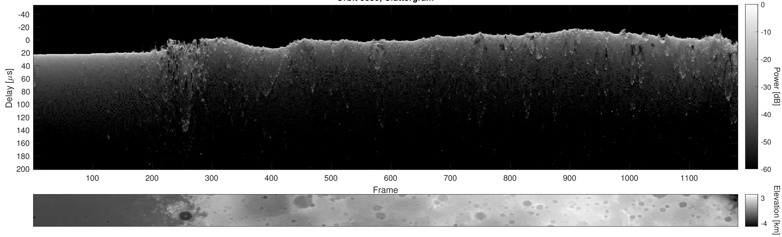
Orbit 9350, Cluttergram
