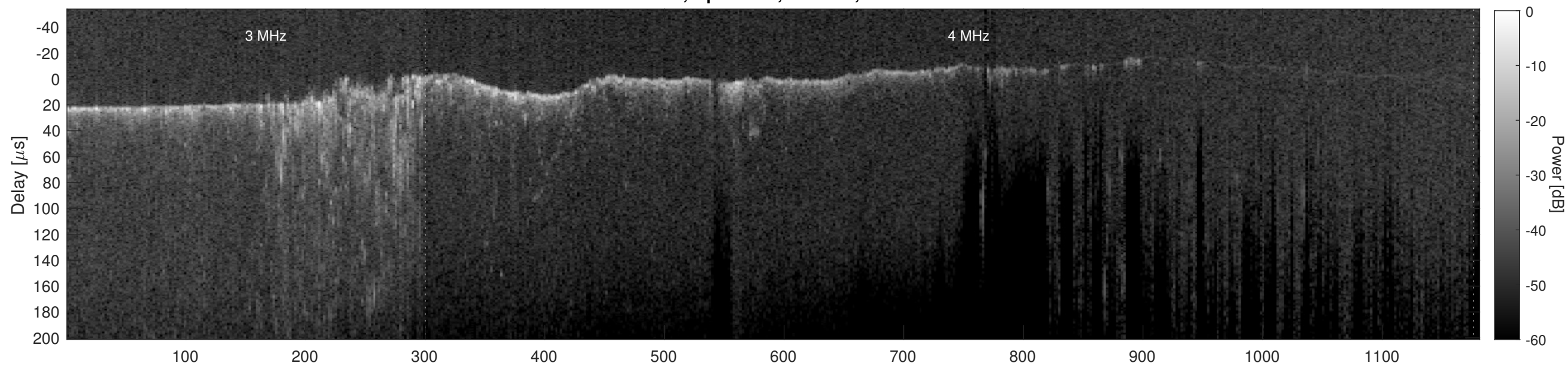
Orbit 9350, Cluttergram
