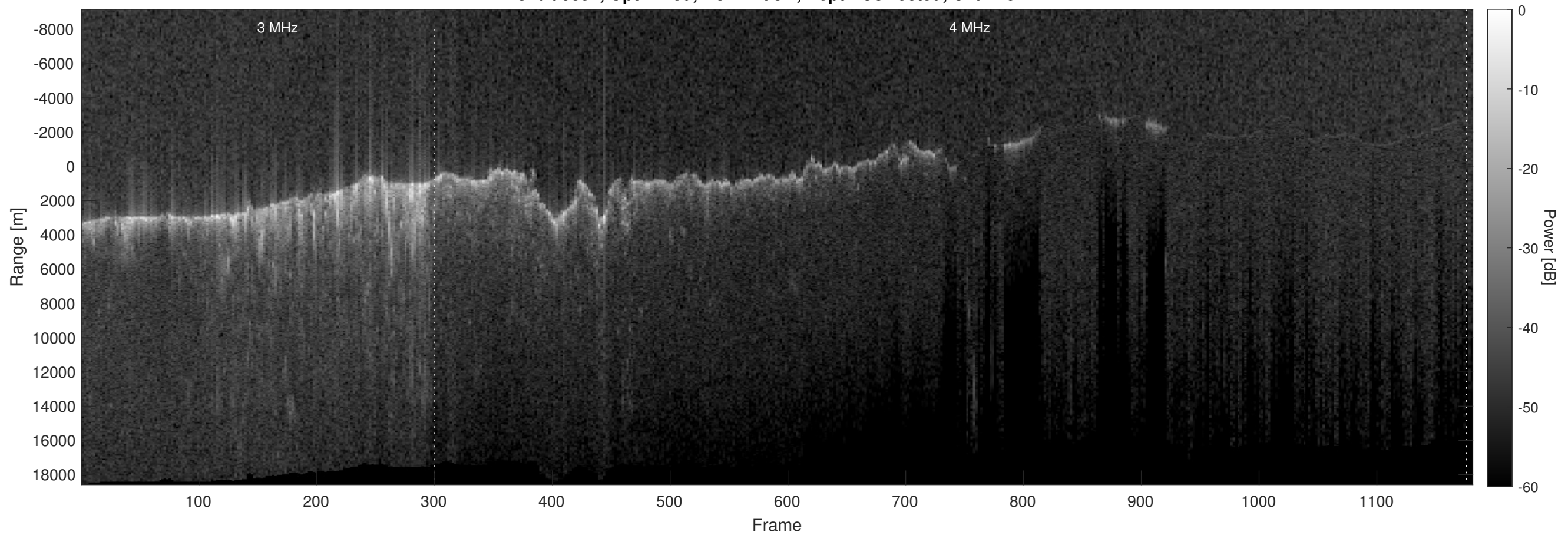
Orbit 9351, Optimized, No Window, Depth-Corrected, Channel 2
