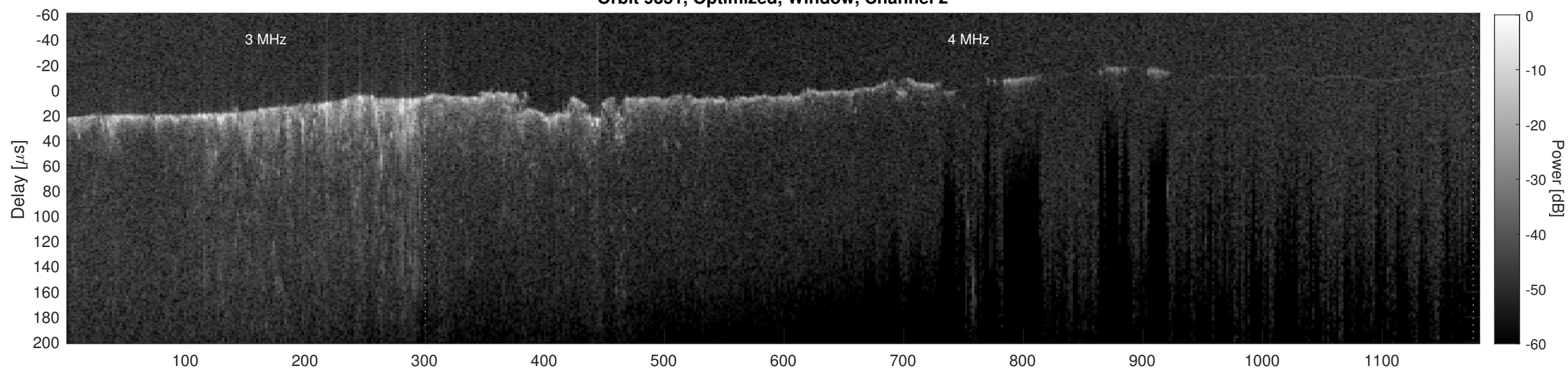
Orbit 9351, Cluttergram
