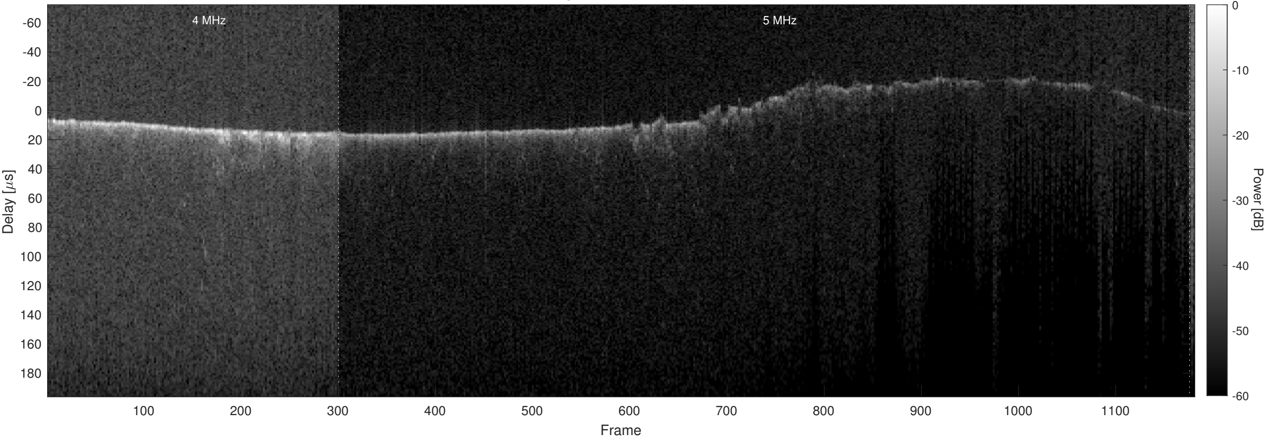
Orbit 9353, Optimized, Window, Channel 2
