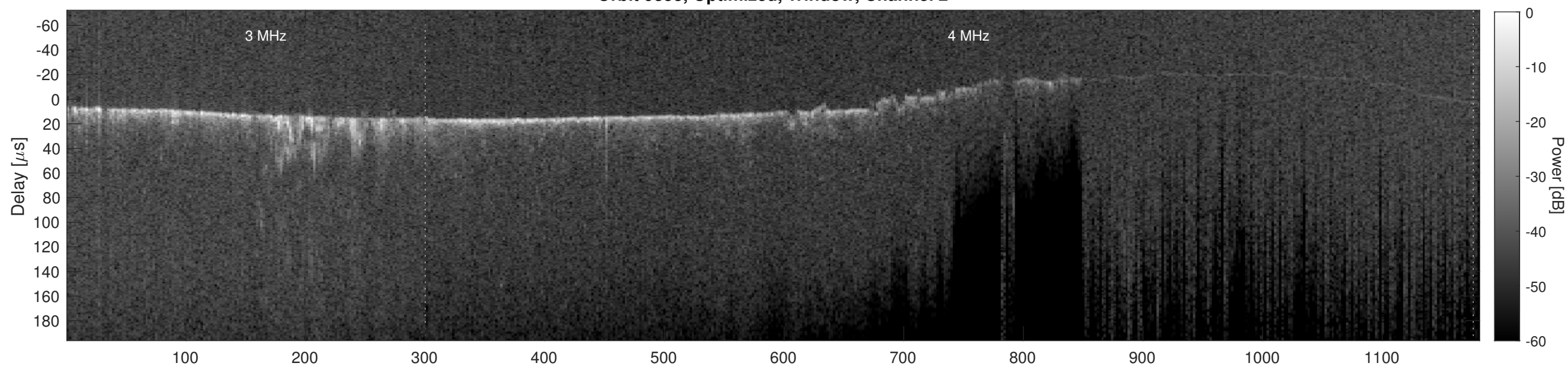
Orbit 9353, Cluttergram
