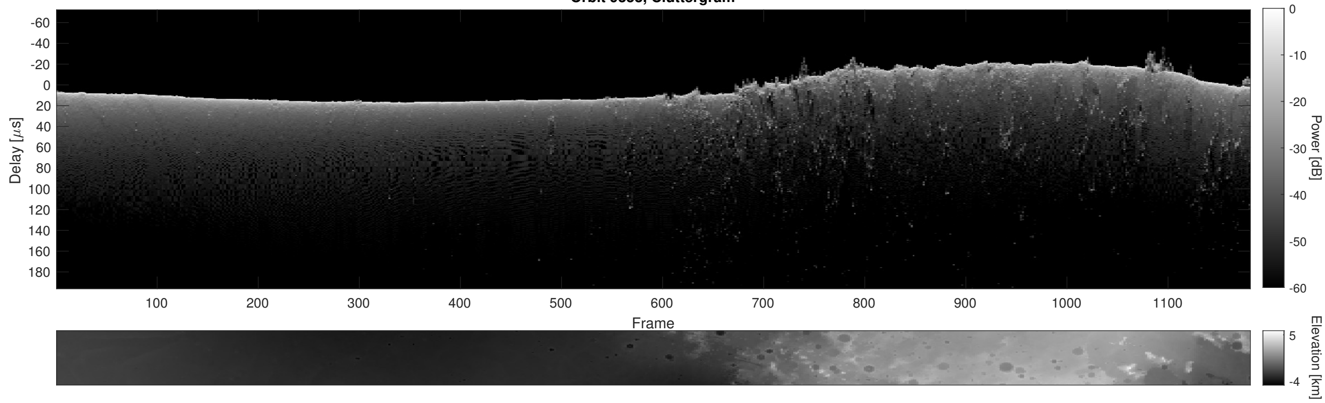
Orbit 9353, Cluttergram
