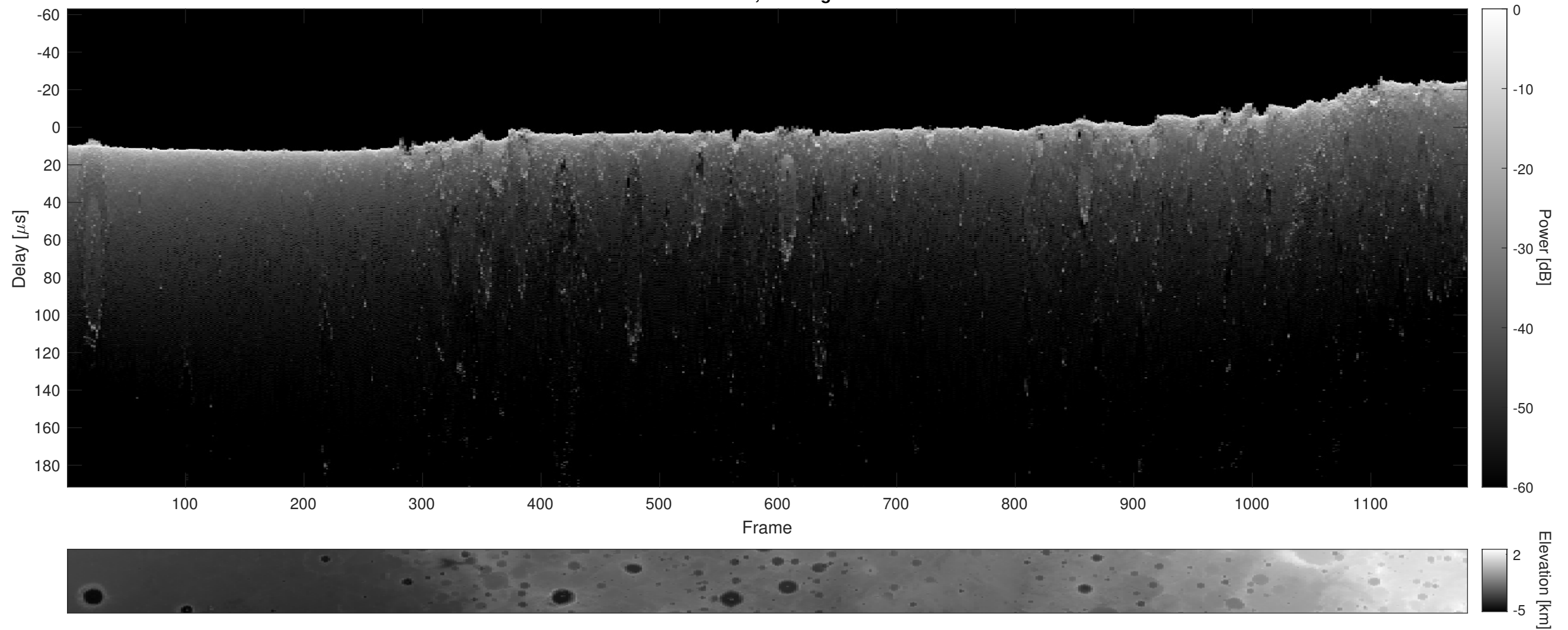
Orbit 9354, Cluttergram
