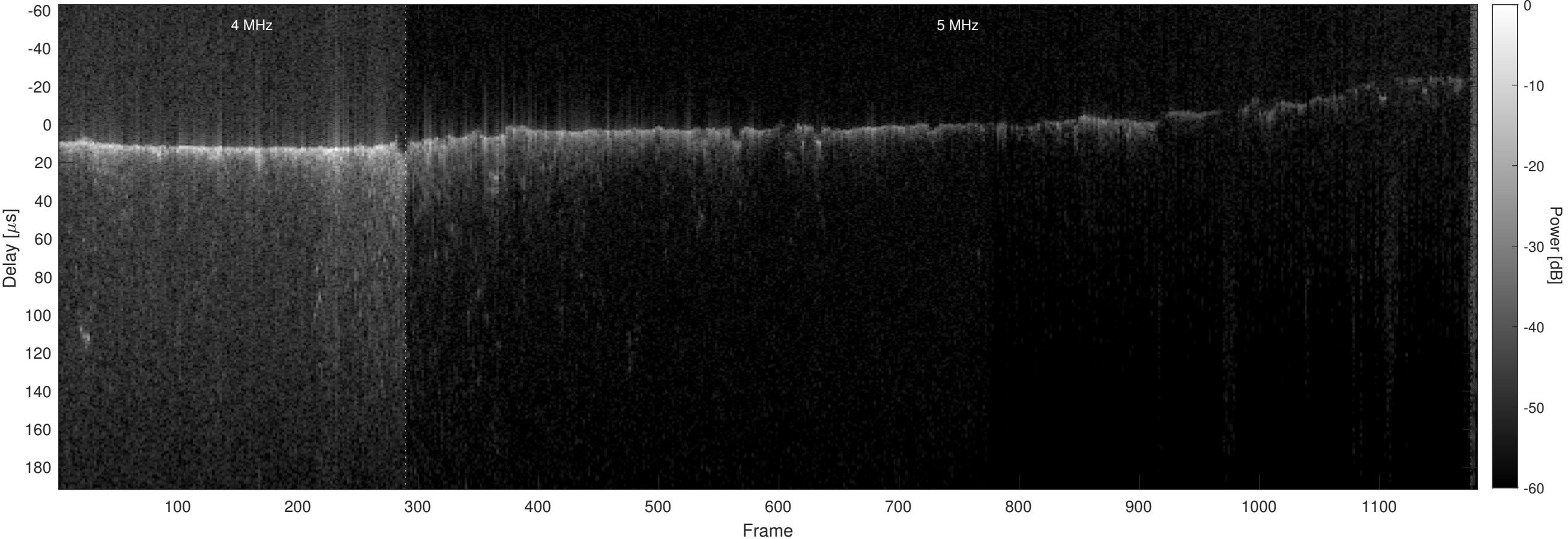
Orbit 9354, Optimized, No Window, Channel 2
