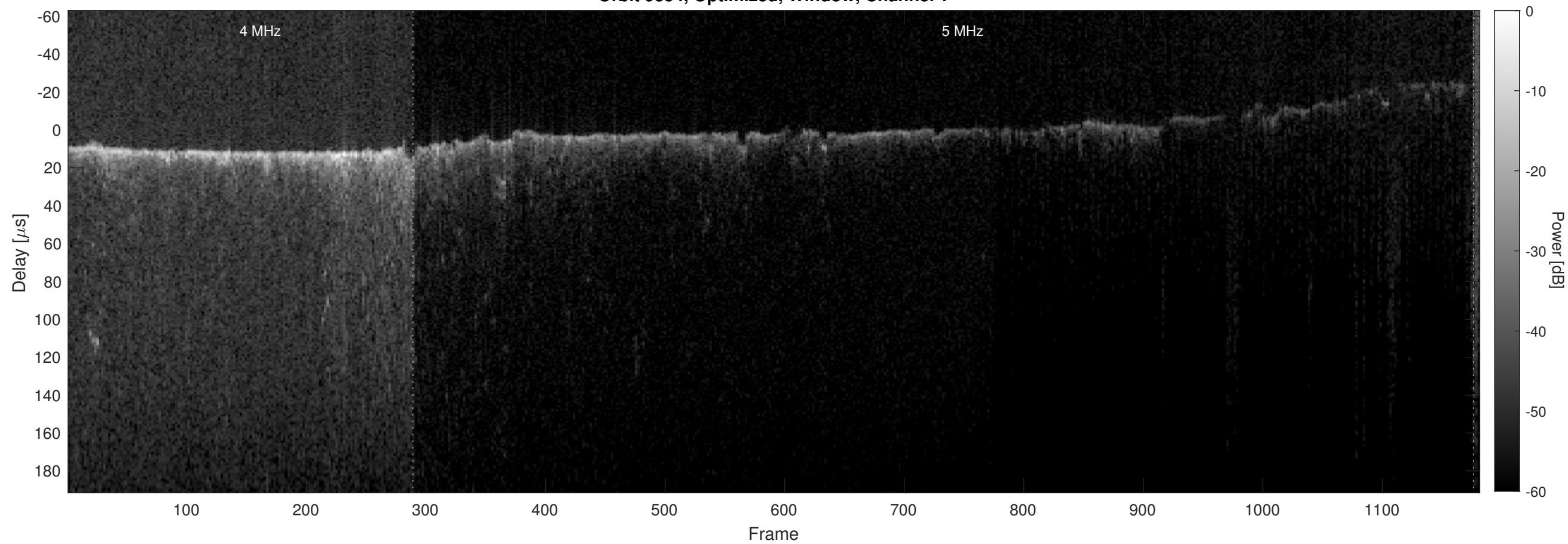
Orbit 9354, Optimized, Window, Channel 2
