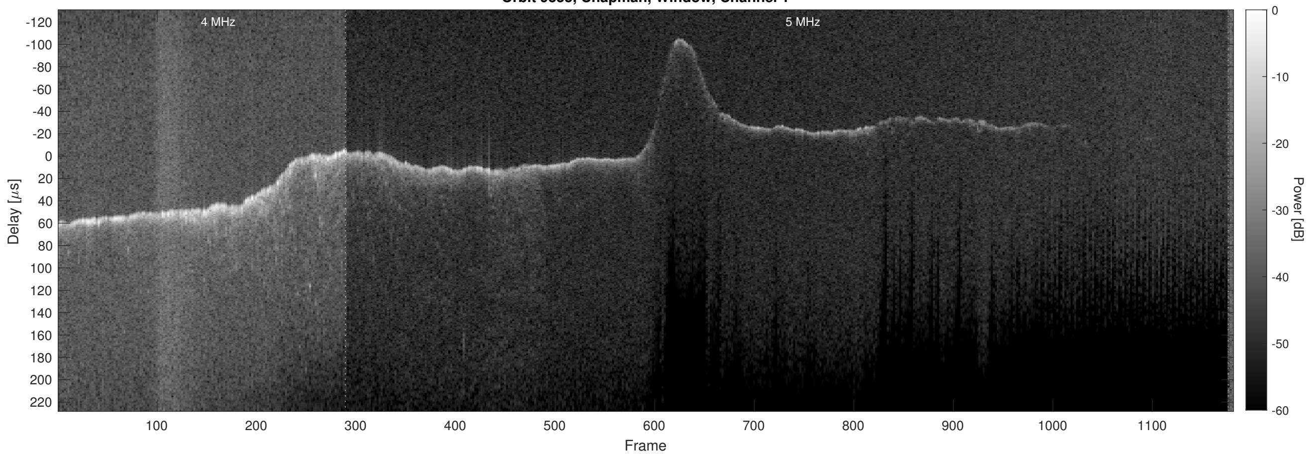
Orbit 9355, Chapman, Window, Channel 2
