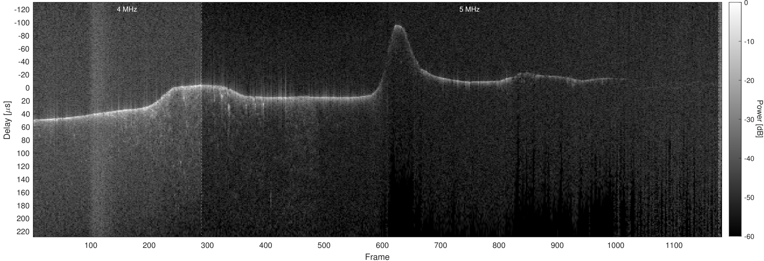
Orbit 9355, Optimized, No Window, Channel 2
