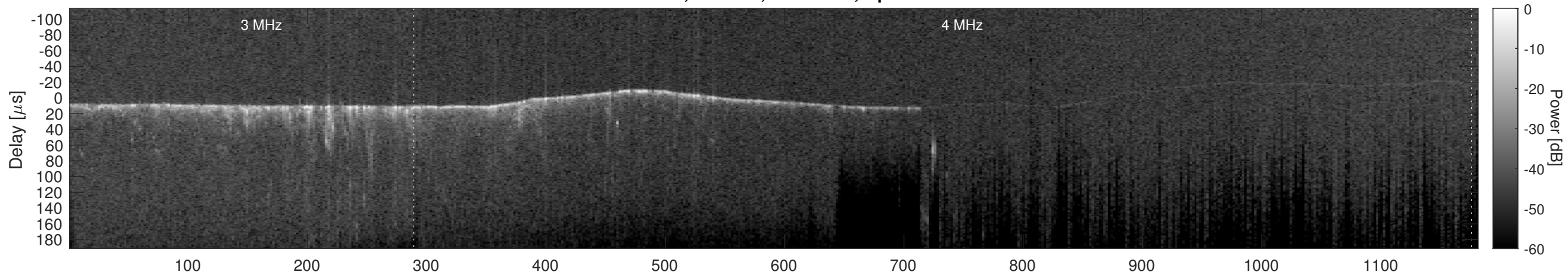
Orbit 9356, Cluttergram
