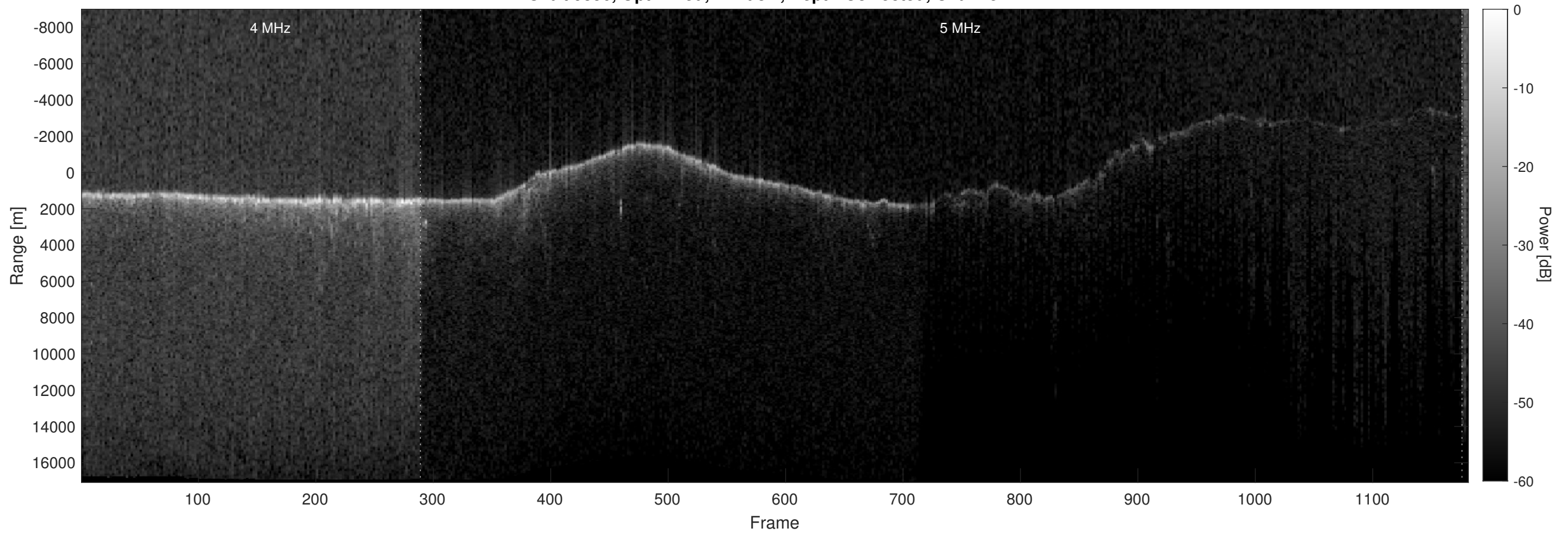
Orbit 9356, Optimized, Window, Depth-Corrected, Channel 2
