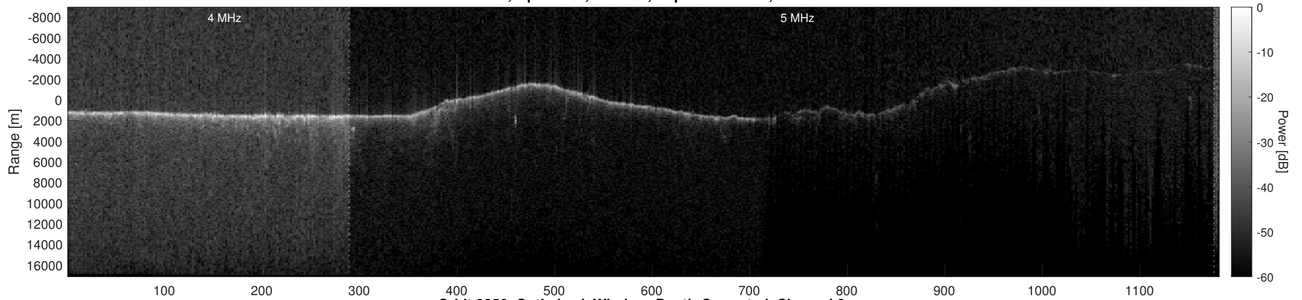
Orbit 9356, Optimized, Window, Depth-Corrected, Channel 2
