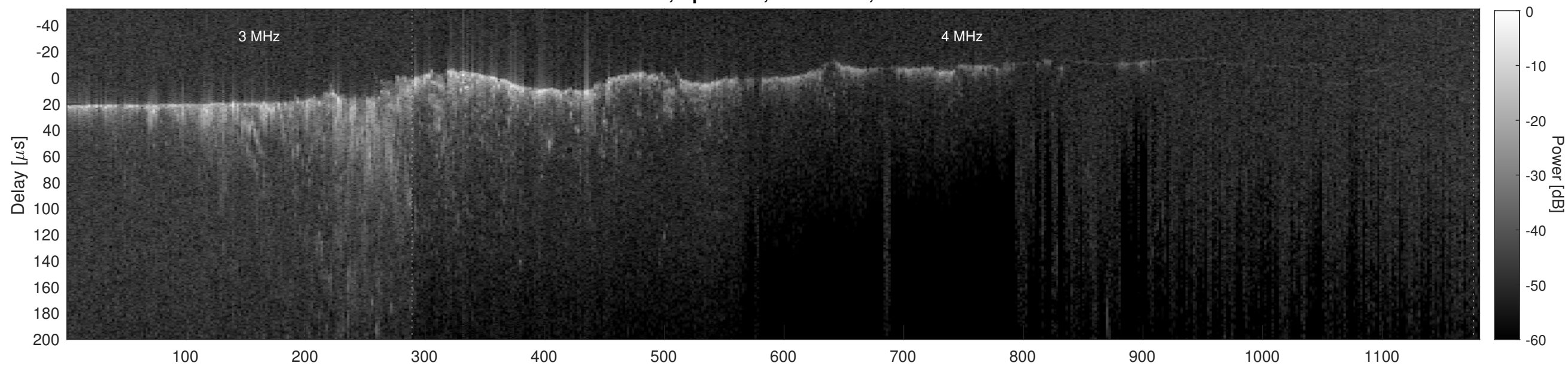
Orbit 9357, Cluttergram
