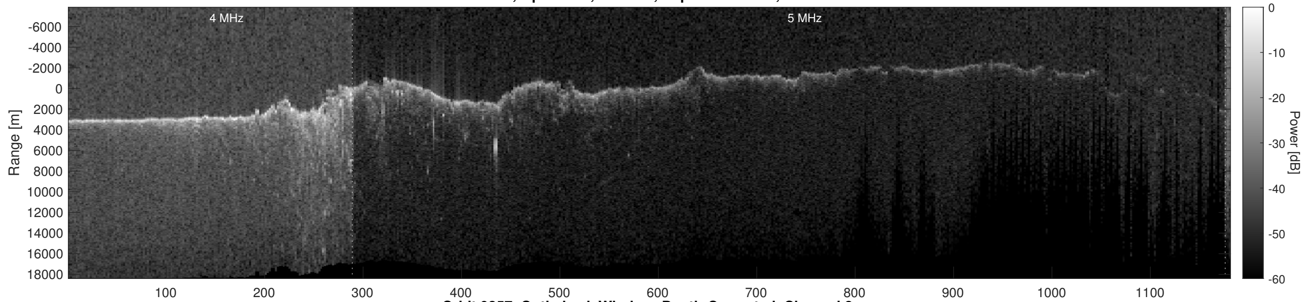
Orbit 9357, Optimized, Window, Depth-Corrected, Channel 2
