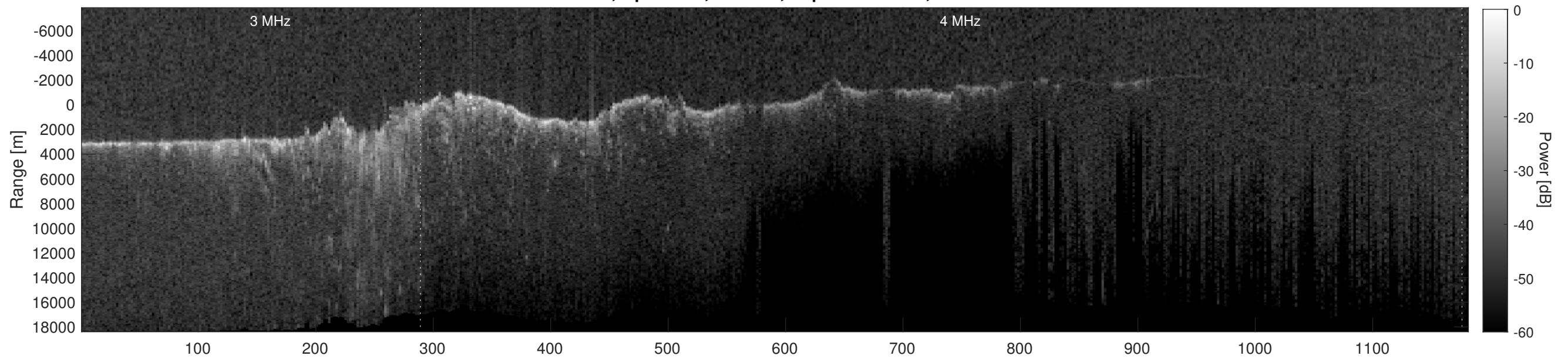
Orbit 9357, Depth-Corrected Cluttergram
