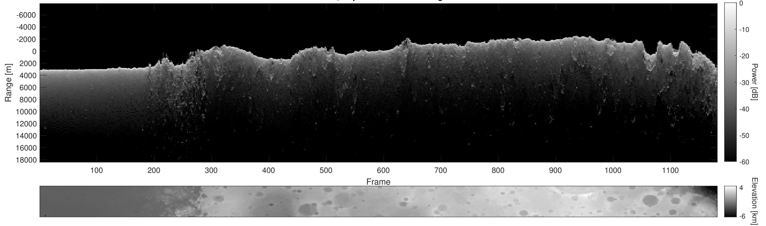
Orbit 9357, Depth-Corrected Cluttergram
