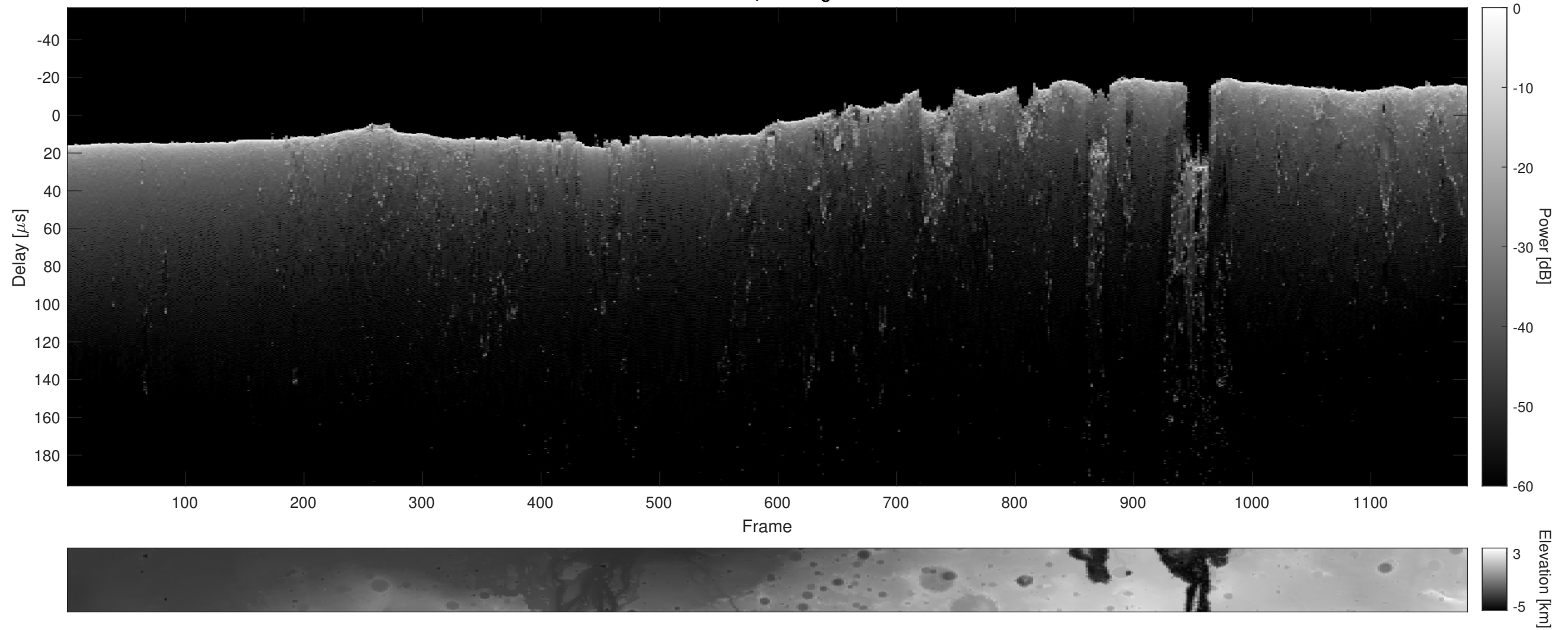
Orbit 9358, Cluttergram
