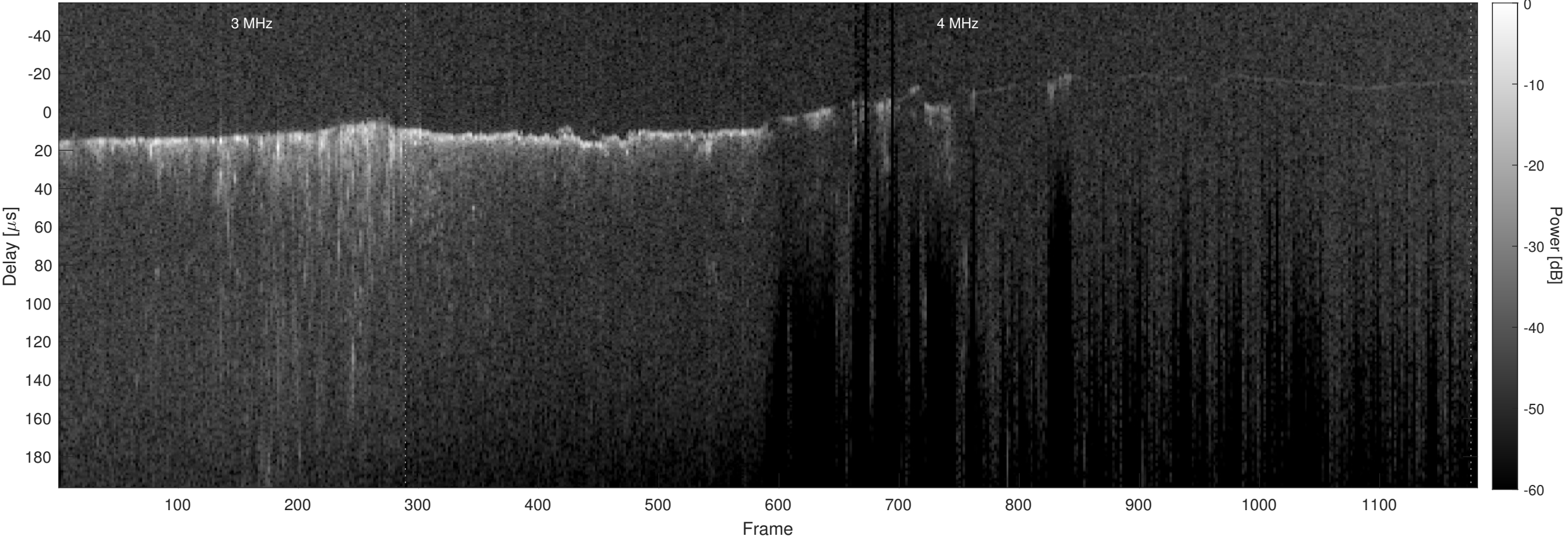
Orbit 9358, Optimized, Window, Channel 2
