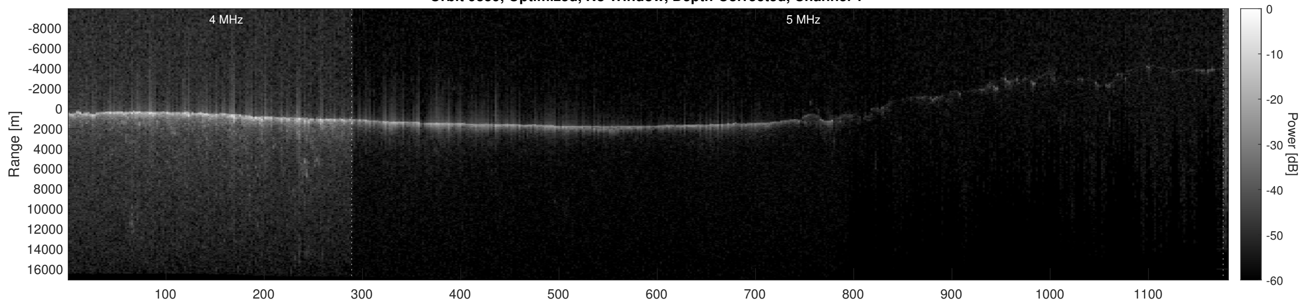
Orbit 9359, Optimized, No Window, Depth-Corrected, Channel 2
