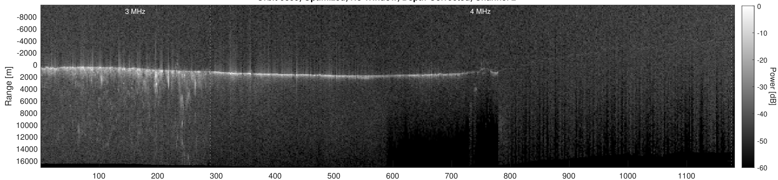
Orbit 9359, Depth-Corrected Cluttergram
