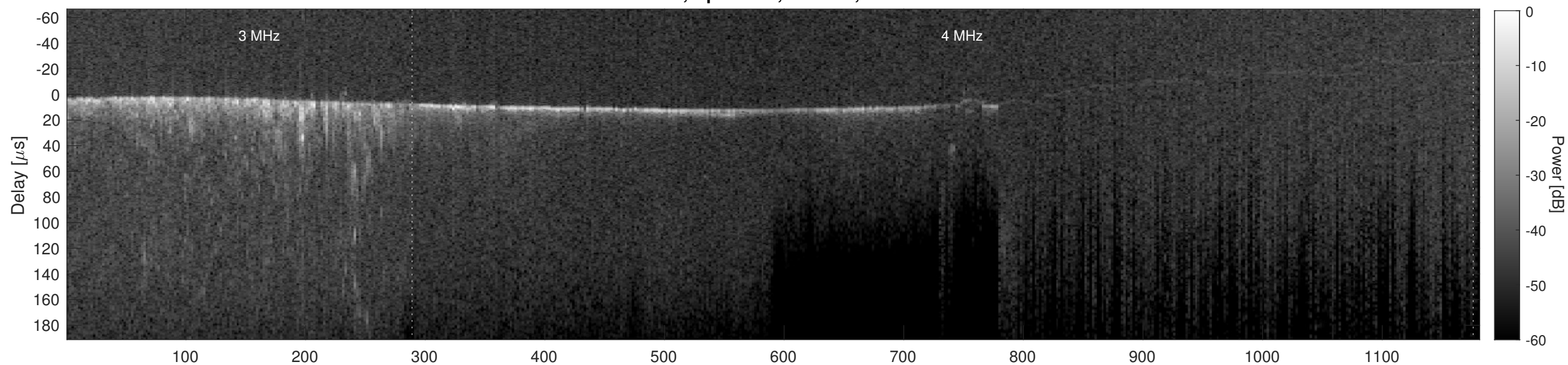
Orbit 9359, Cluttergram
