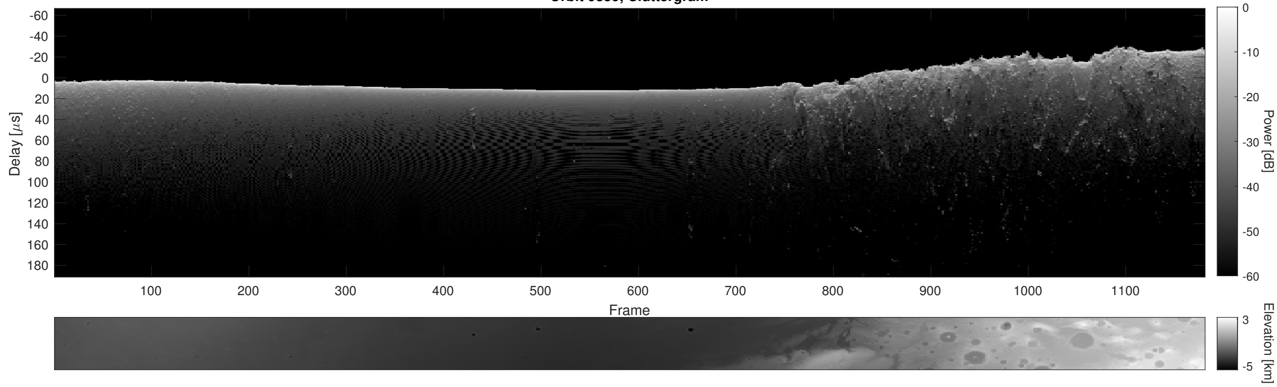
Orbit 9359, Cluttergram
