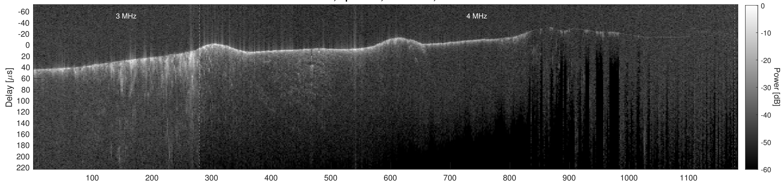
Orbit 9362, Cluttergram
