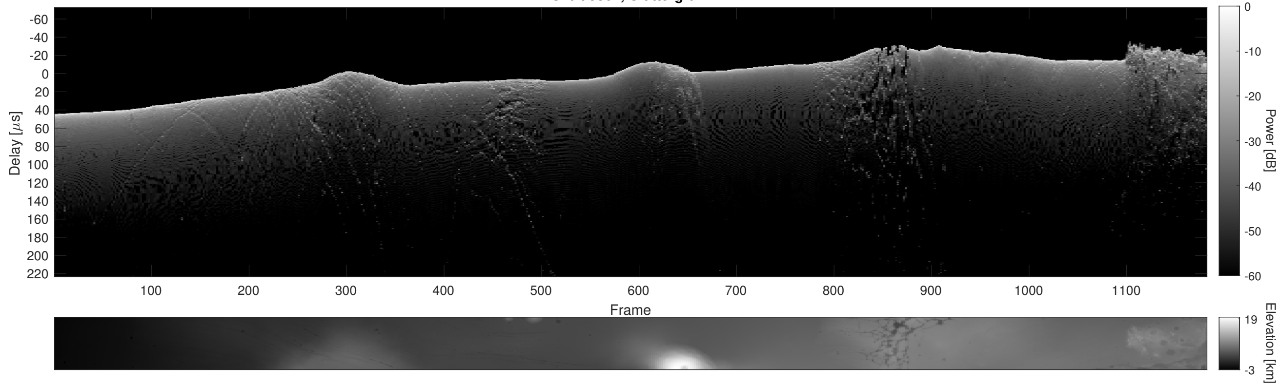
Orbit 9362, Cluttergram
