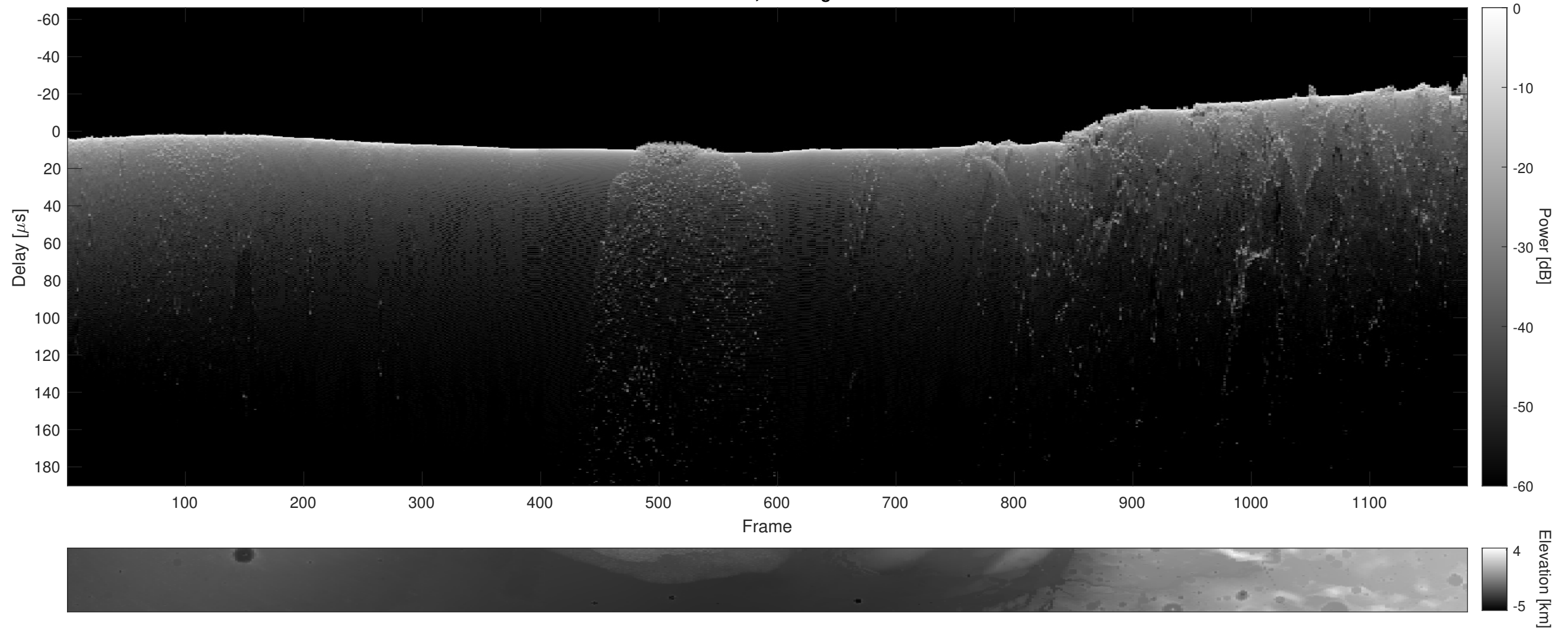
Orbit 9366, Cluttergram
