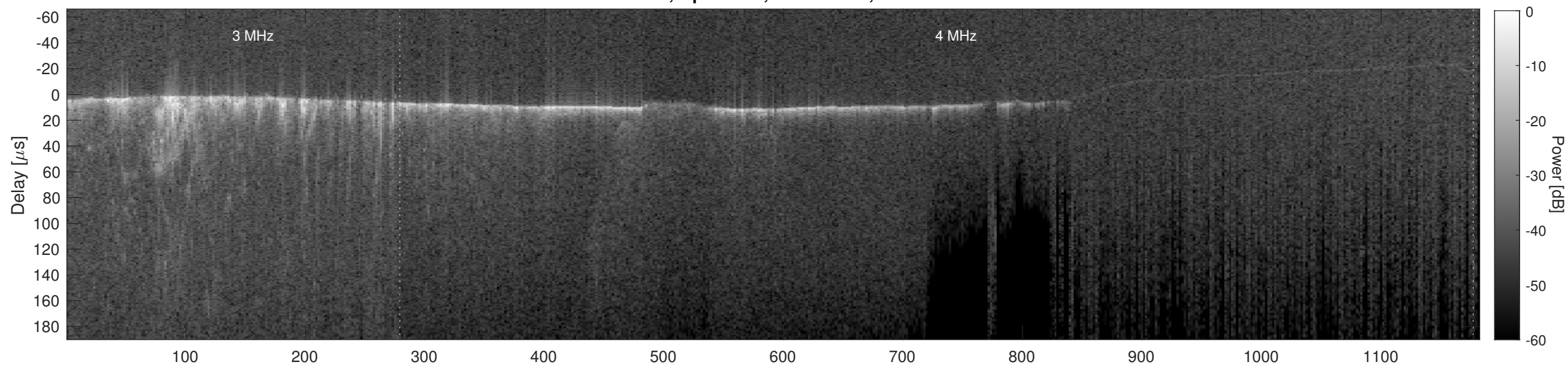
Orbit 9366, Cluttergram
