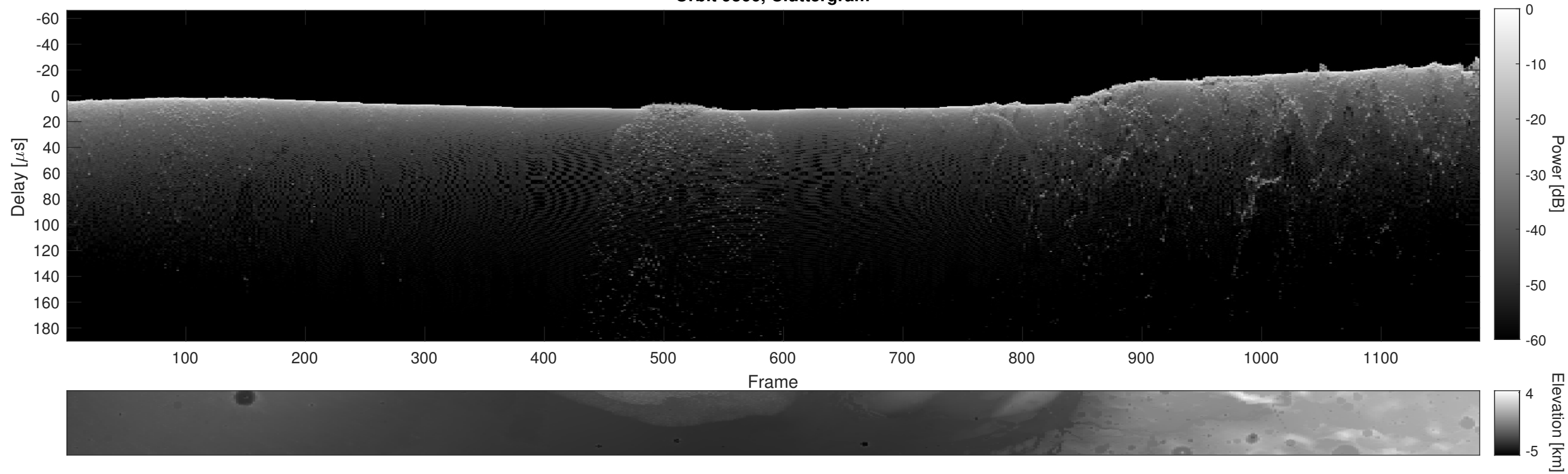
Orbit 9366, Cluttergram
