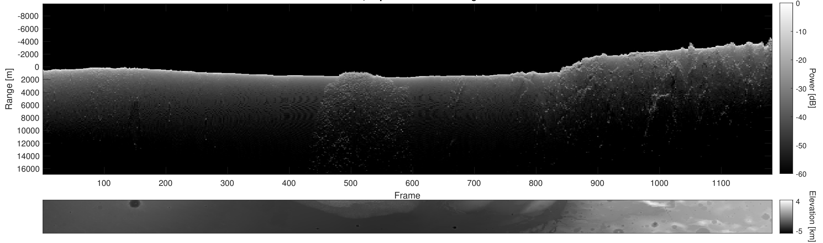
Orbit 9366, Depth-Corrected Cluttergram
