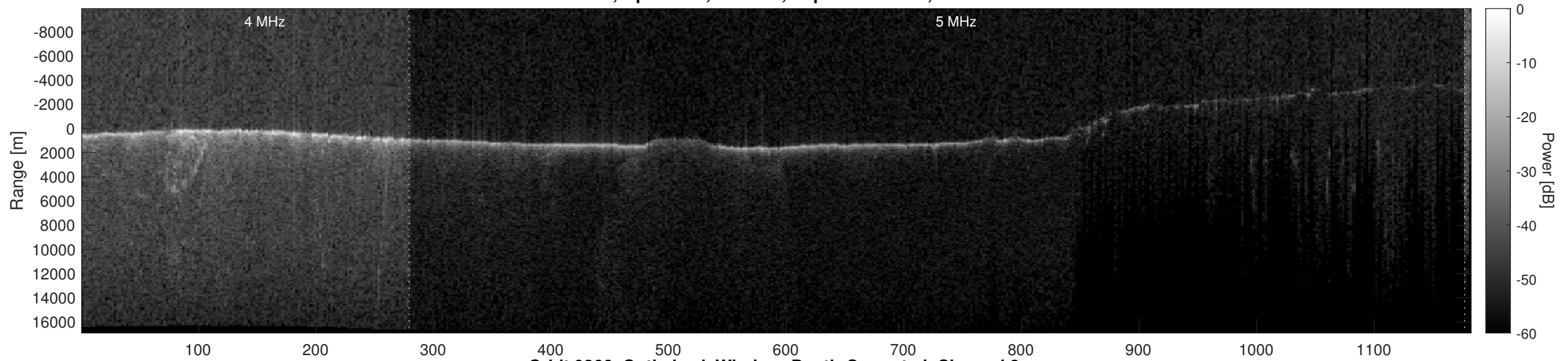
Orbit 9366, Optimized, Window, Depth-Corrected, Channel 2
