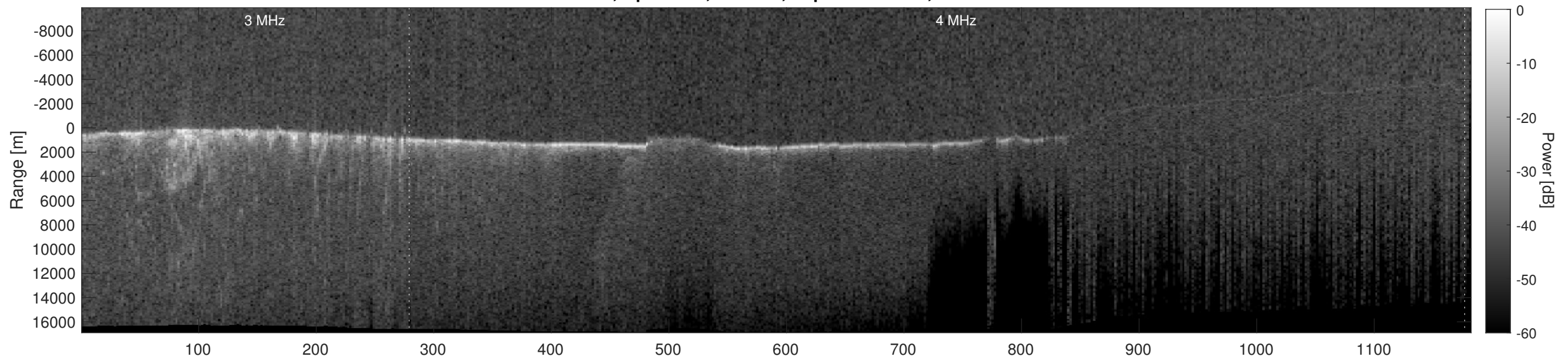
Orbit 9366, Depth-Corrected Cluttergram
