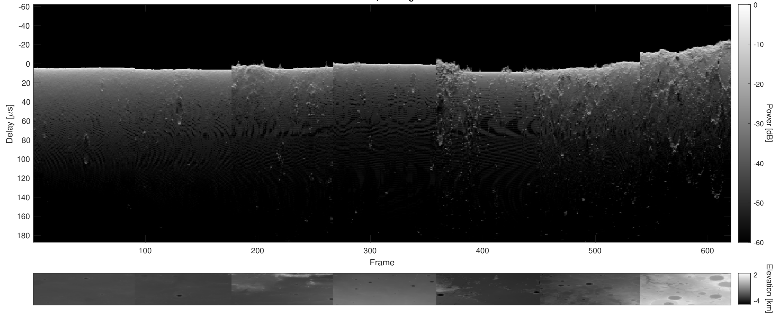
Orbit 9370, Cluttergram
