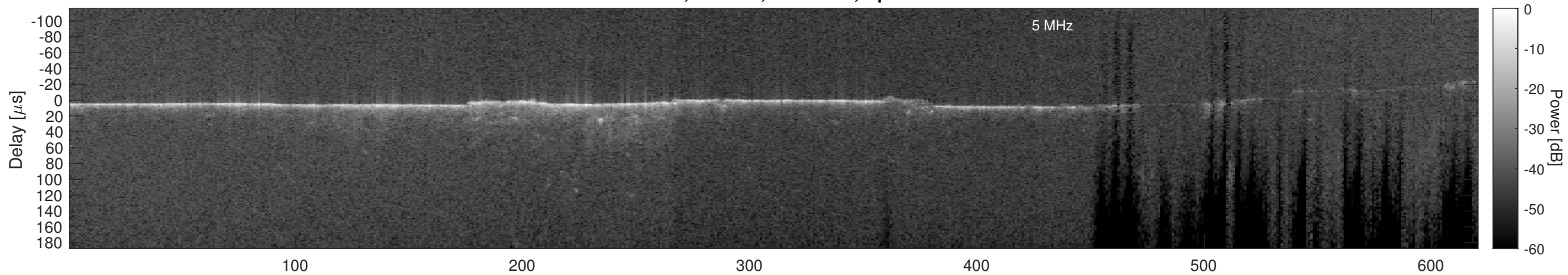
Orbit 9370, Cluttergram
