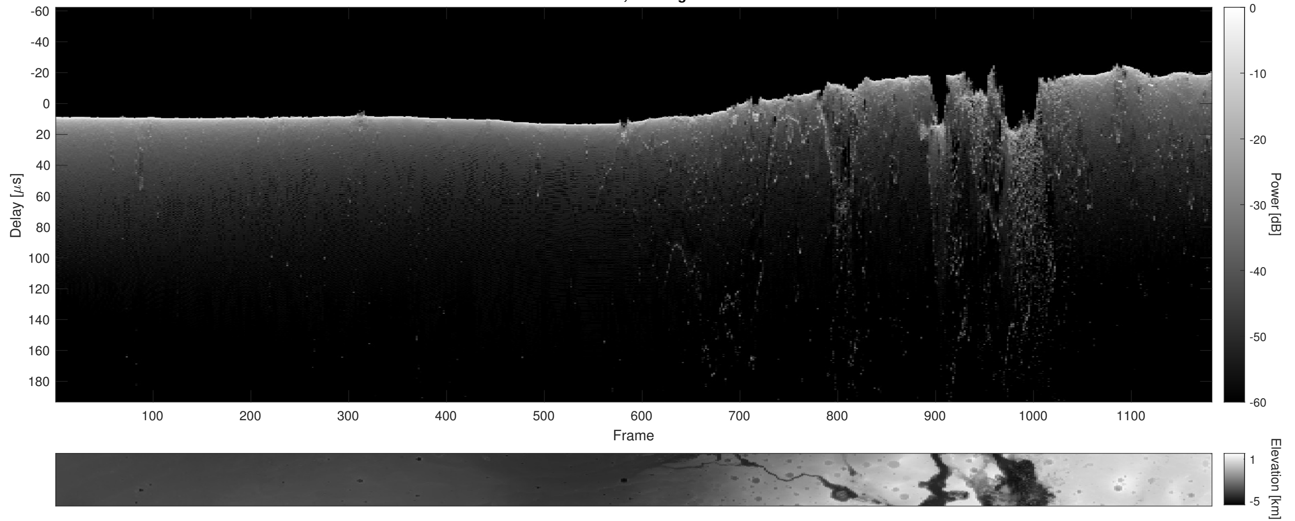
Orbit 9372, Cluttergram
