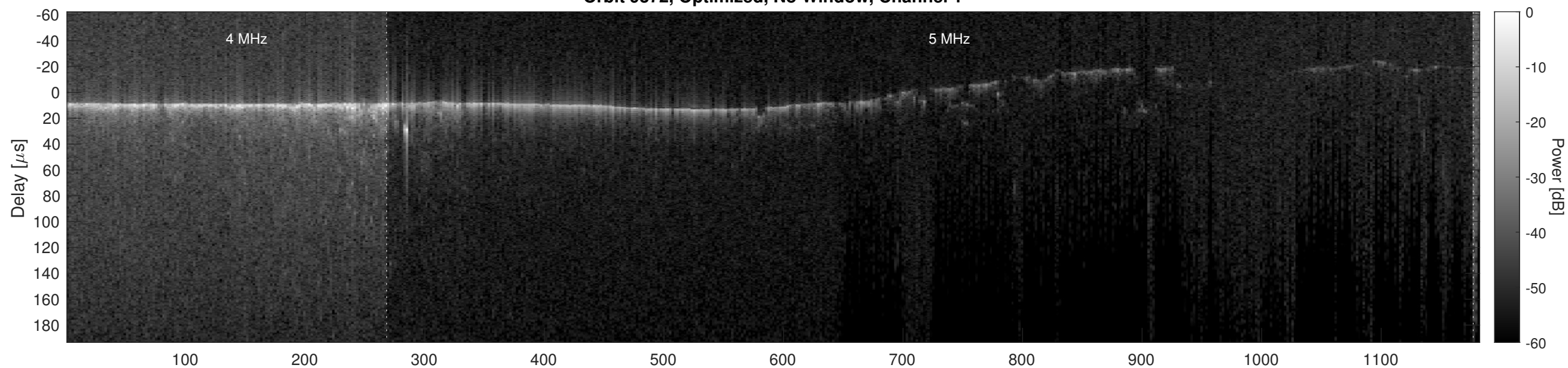
Orbit 9372, Optimized, No Window, Channel 2
