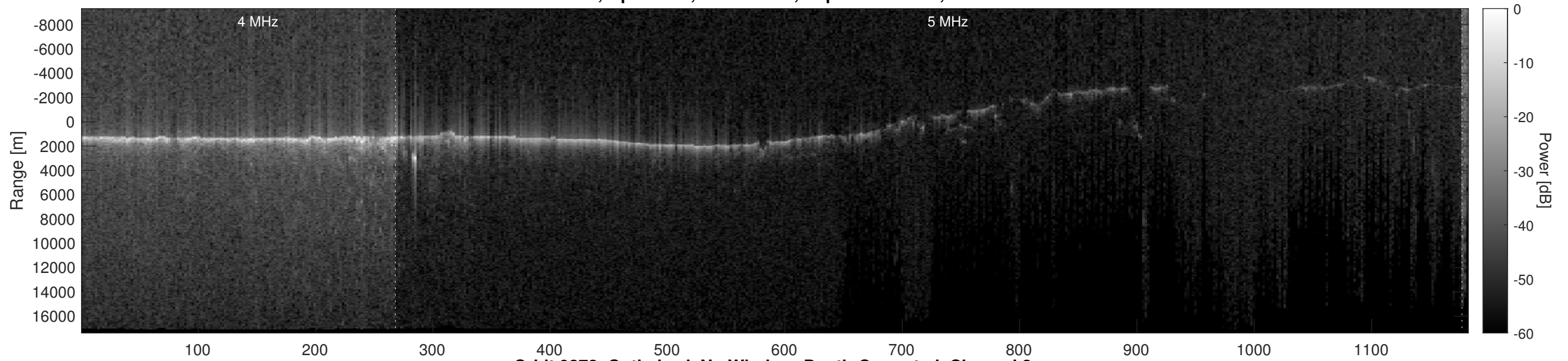
Orbit 9372, Optimized, No Window, Depth-Corrected, Channel 2
