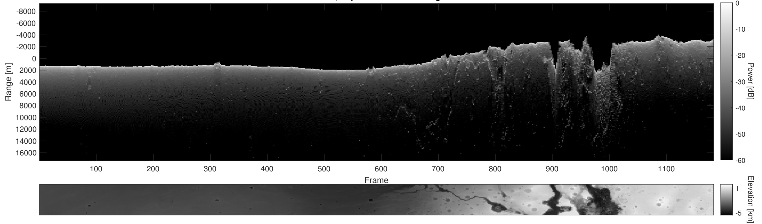
Orbit 9372, Depth-Corrected Cluttergram
