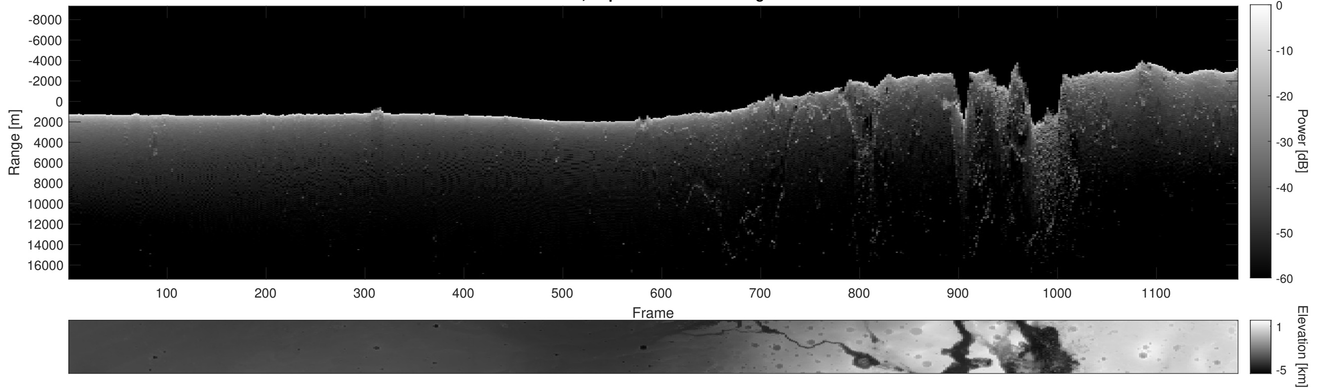
Orbit 9372, Depth-Corrected Cluttergram
