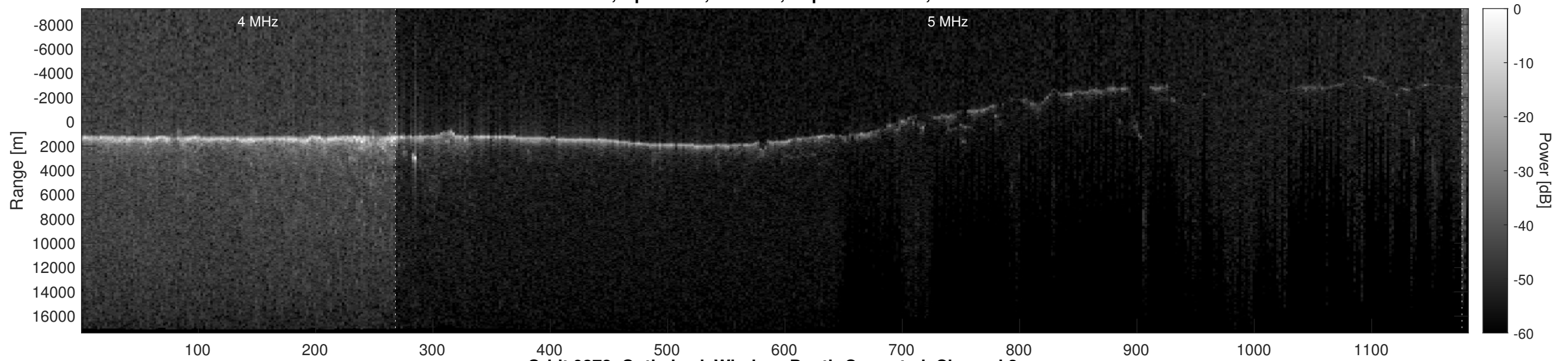
Orbit 9372, Optimized, Window, Depth-Corrected, Channel 2
