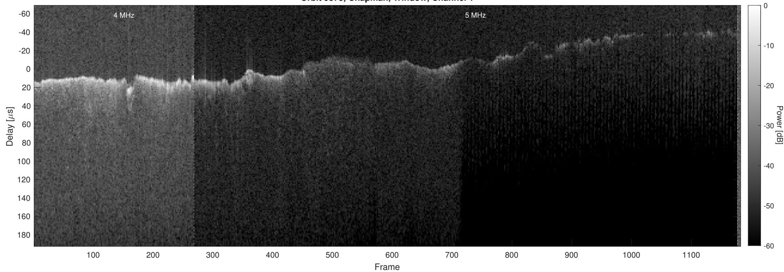
Orbit 9373, Chapman, Window, Channel 2
