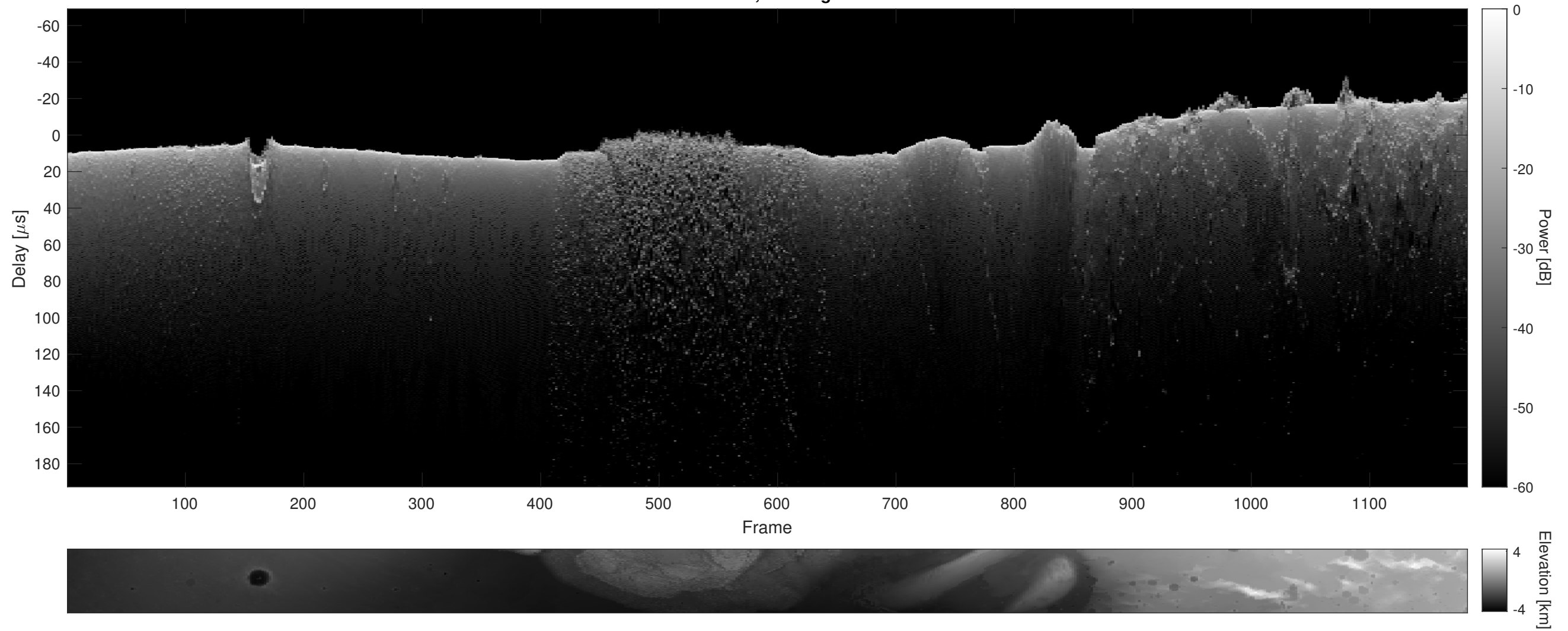
Orbit 9373, Cluttergram
