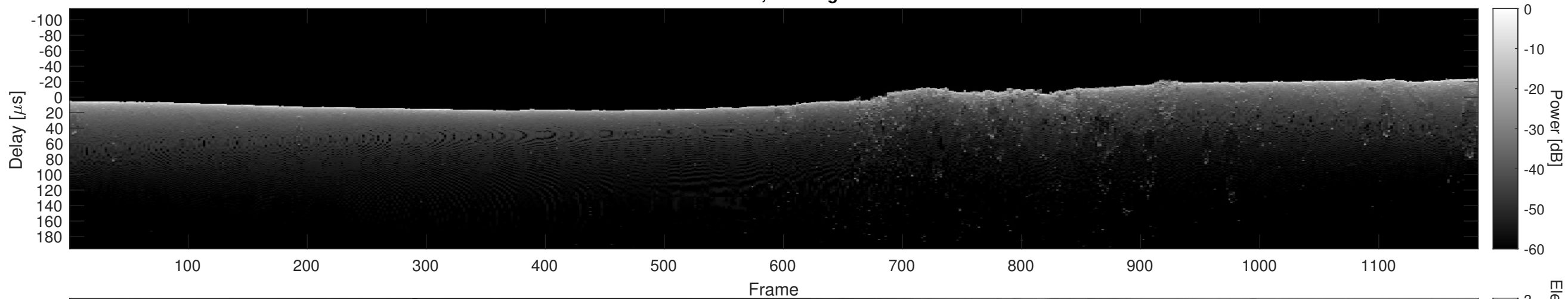
Orbit 9374, Cluttergram
