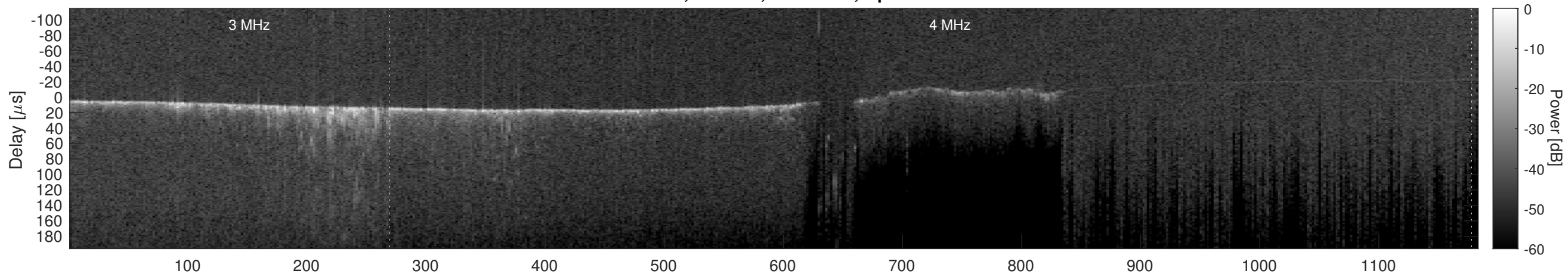
Orbit 9374, Cluttergram
