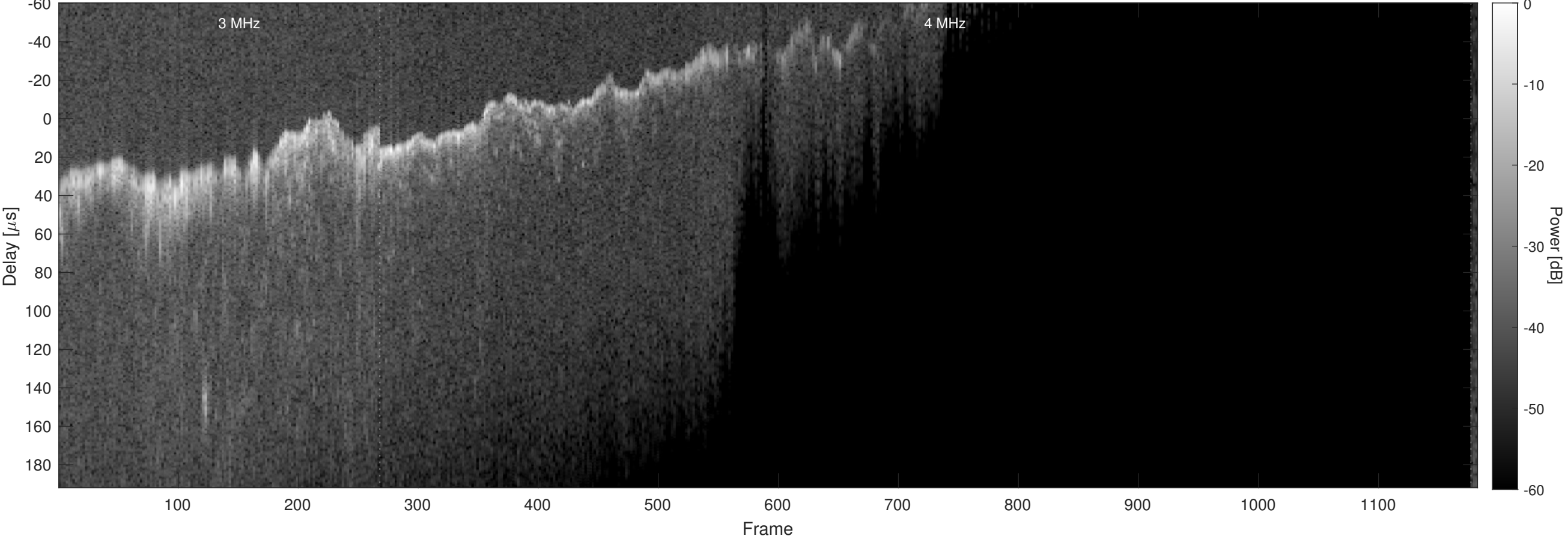
Orbit 9375, Chapman, Window, Channel 2
