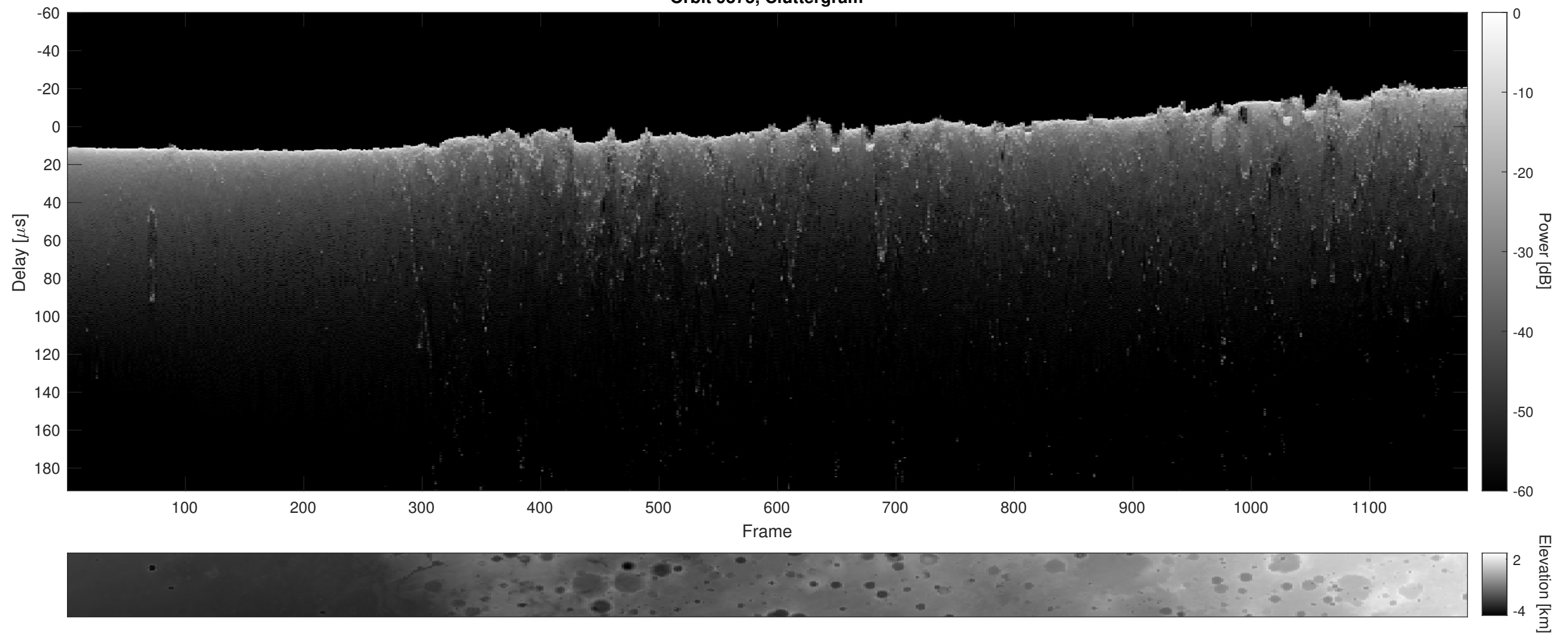
Orbit 9375, Cluttergram
