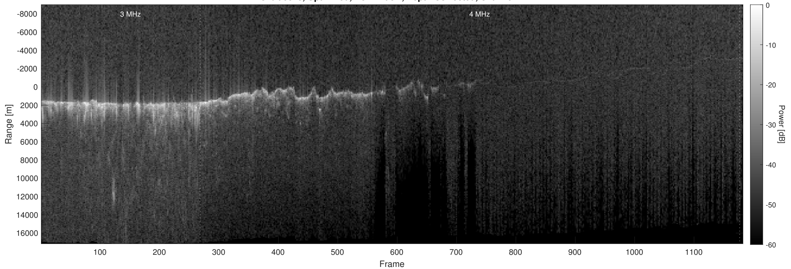
Orbit 9375, Optimized, No Window, Depth-Corrected, Channel 2
