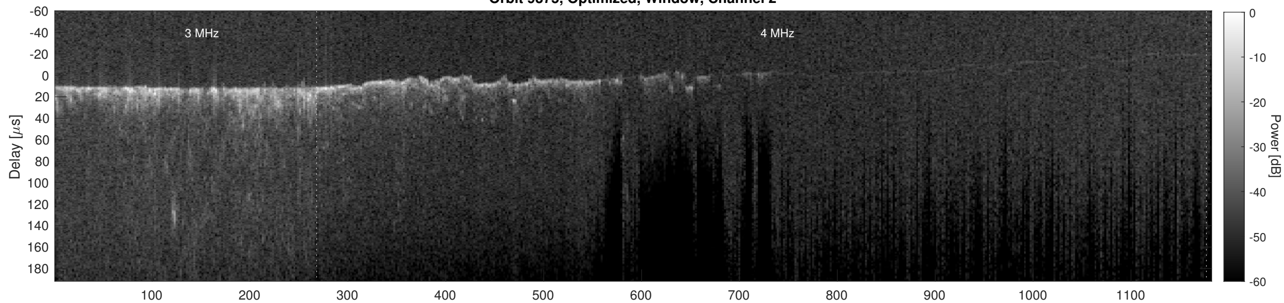
Orbit 9375, Cluttergram
