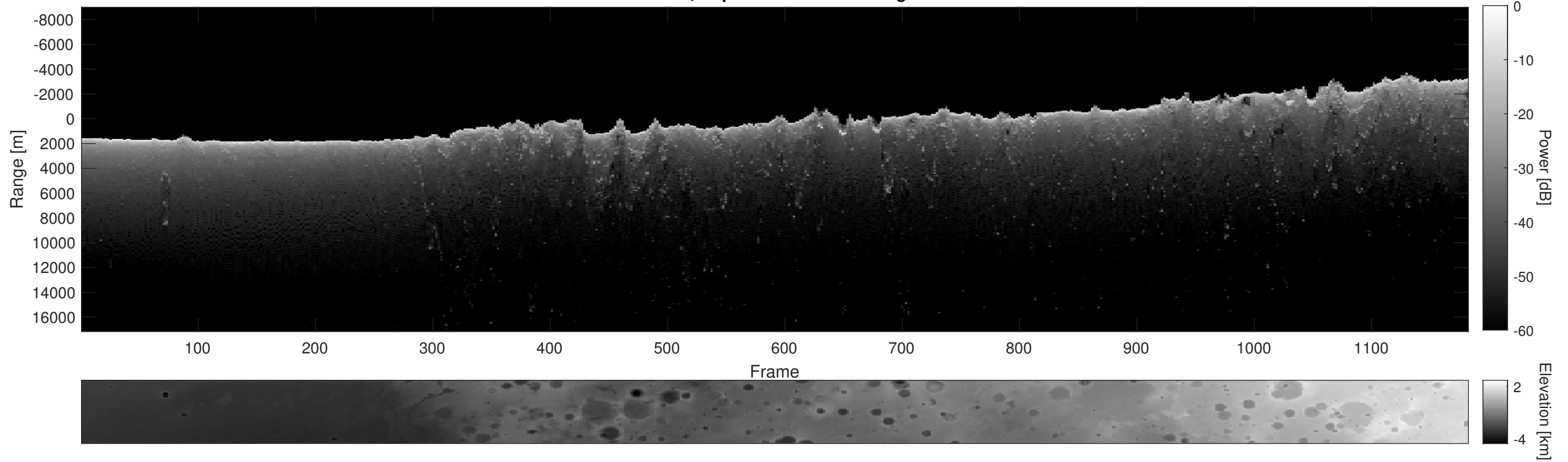
Orbit 9375, Depth-Corrected Cluttergram
