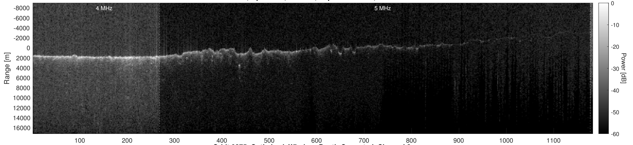
Orbit 9375, Optimized, Window, Depth-Corrected, Channel 2
