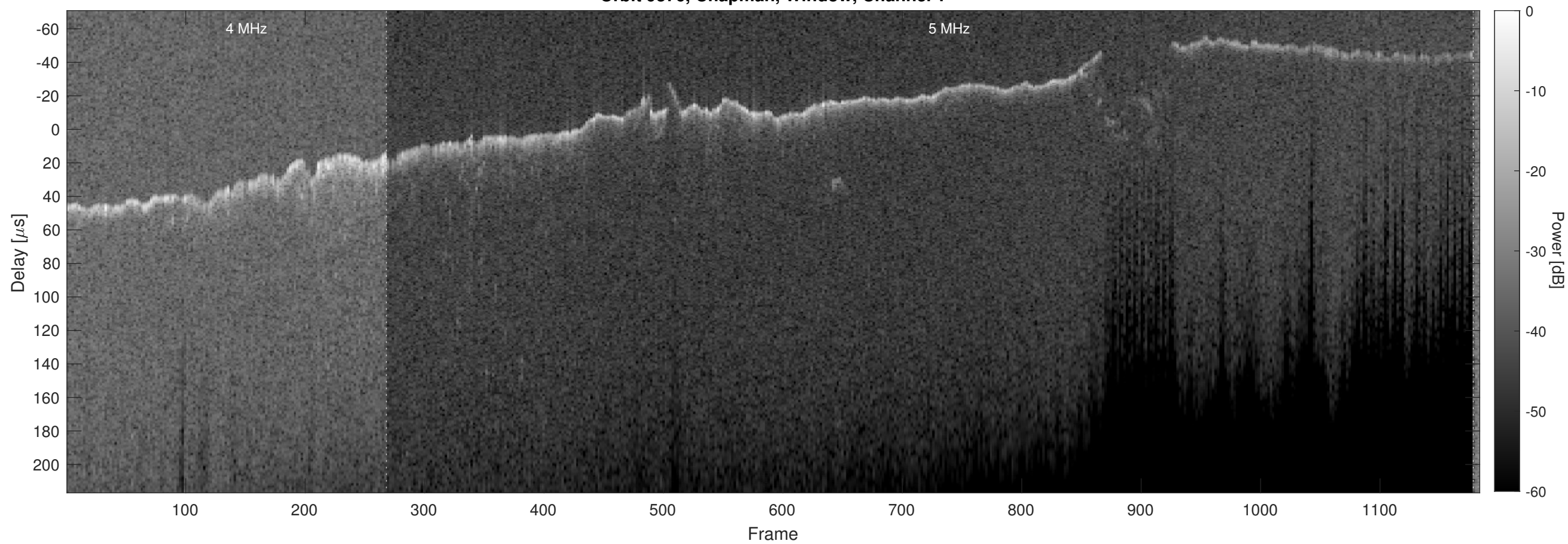
Orbit 9376, Chapman, Window, Channel 2
