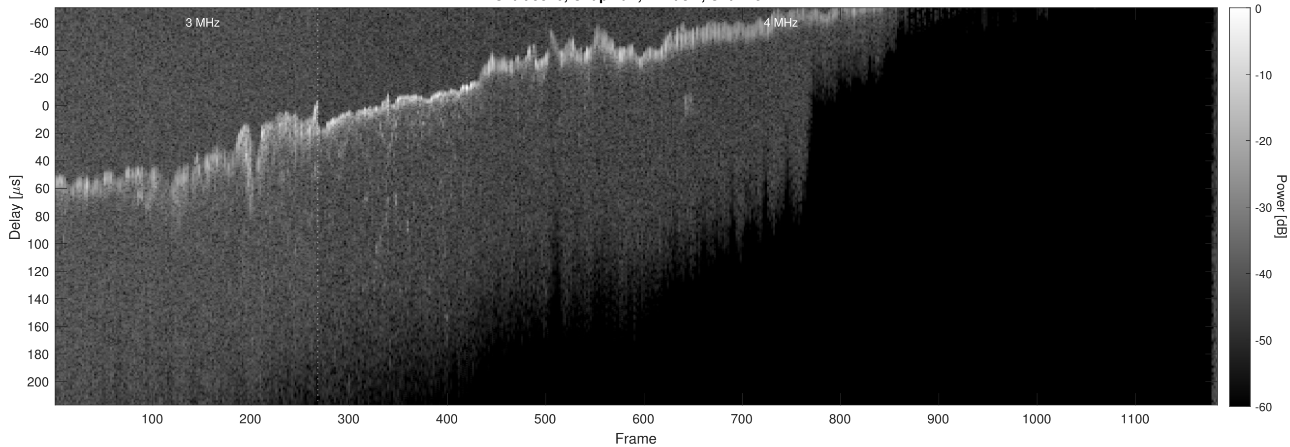
Orbit 9376, Chapman, Window, Channel 2
