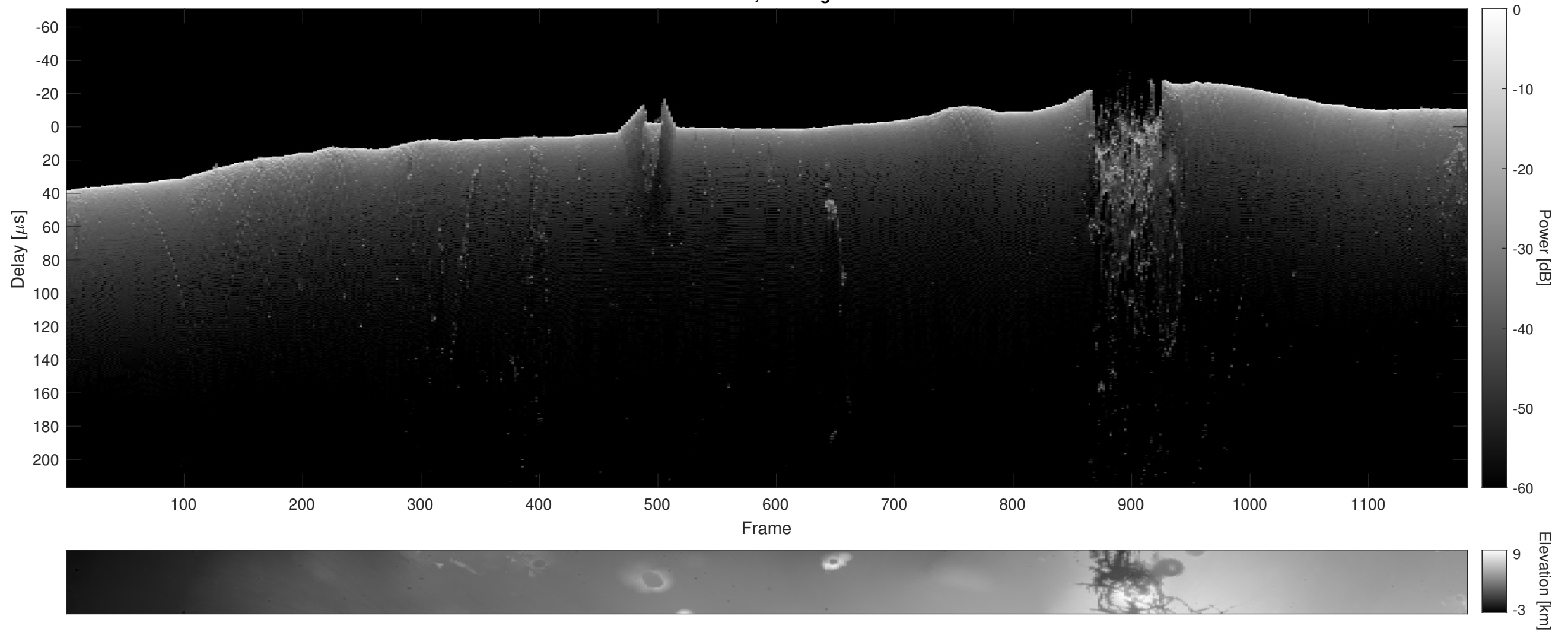
Orbit 9376, Cluttergram
